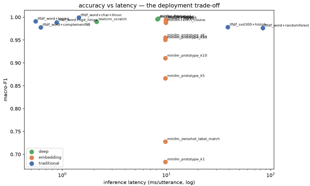
Figure B: Accuracy against inference latency.
