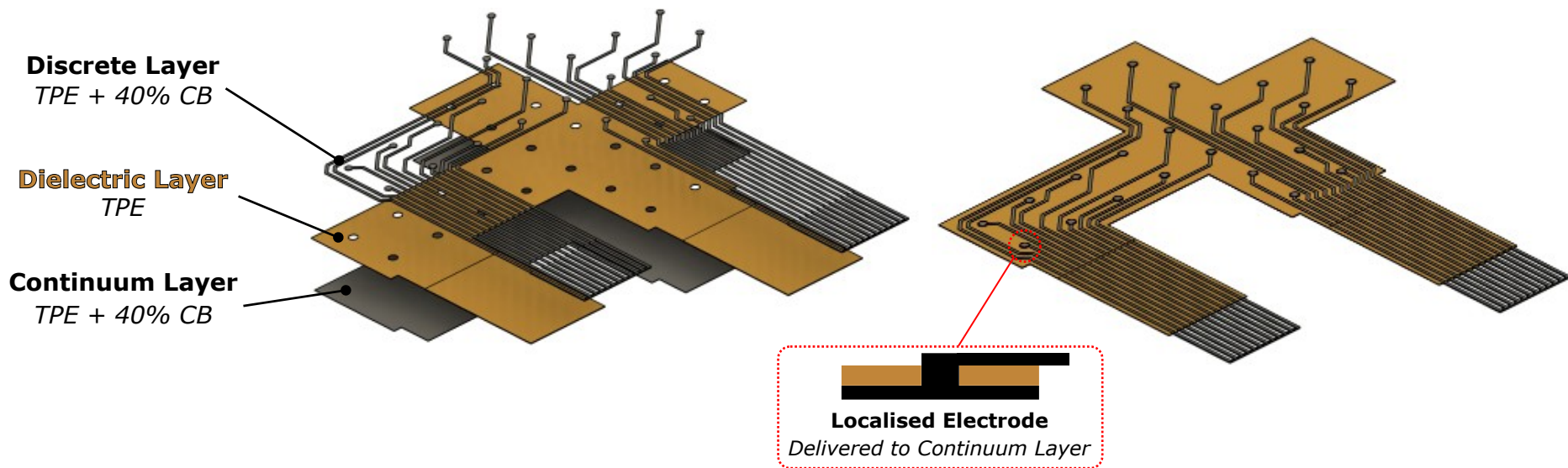
6 Electrode Layout
