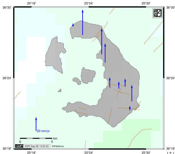
Vertical velocities 20250303 - 20250908 [IGS20]
