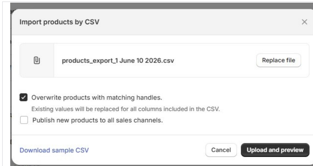
Figure 12 — Shopify import settings dialog with required options.
