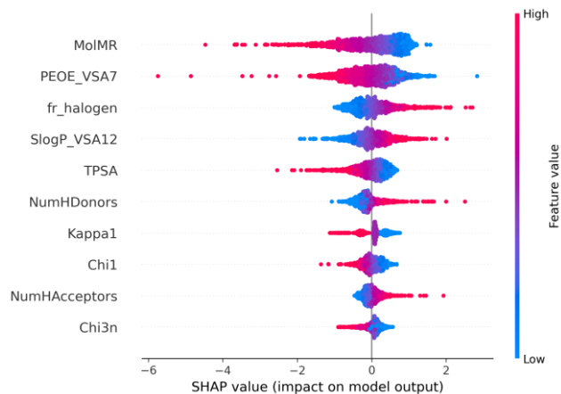
(b) Solubility
