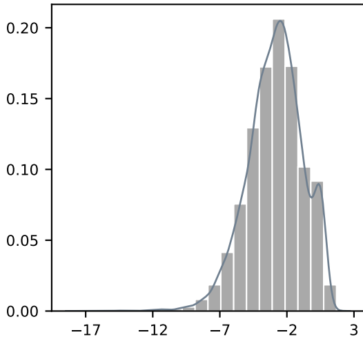
(b) Solubility
