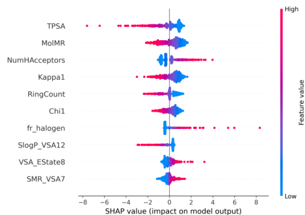
(b) Vapor pressure, Kronecker-product
