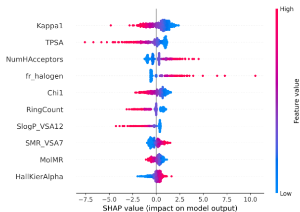
(a) Vapor pressure, Concatenation
