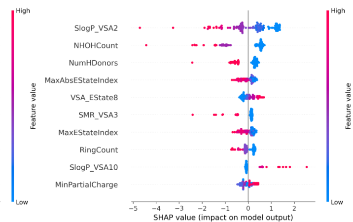
(a) FreeSolv
