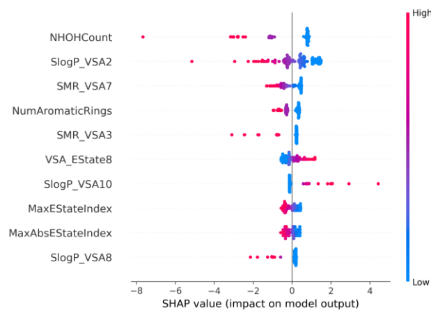
(a) FreeSolv
