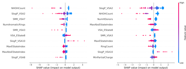
(a) FreeSolv
