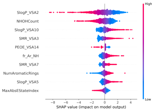
(b) Solubility
