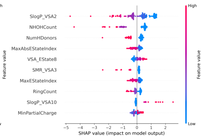
(a) FreeSolv
