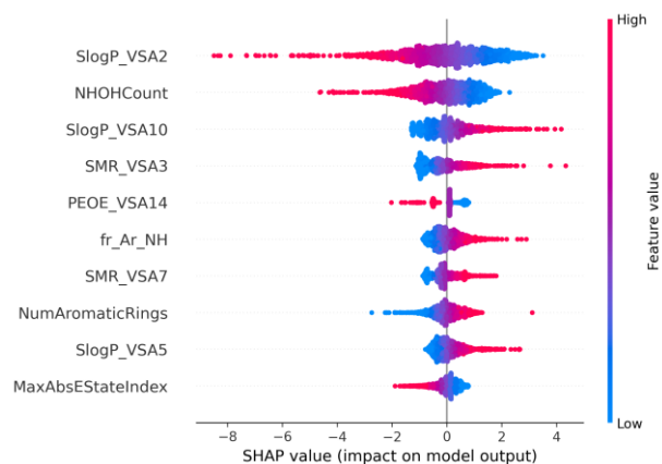
(c) Solubility, Concatenation
