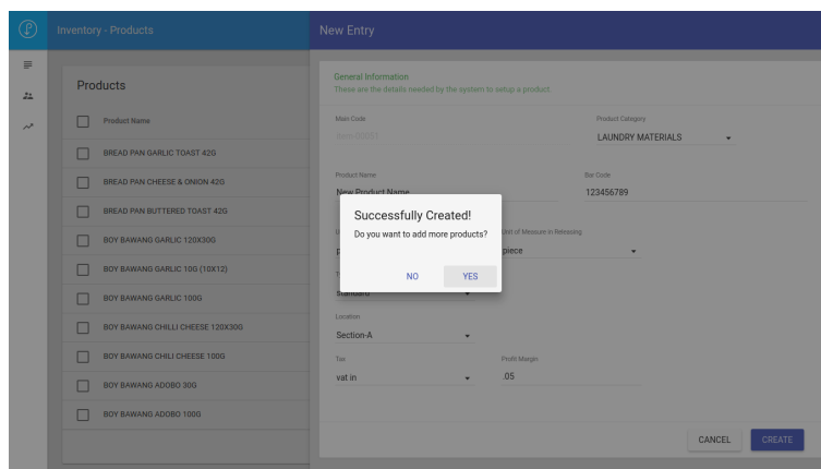
Screenshot 2.0
