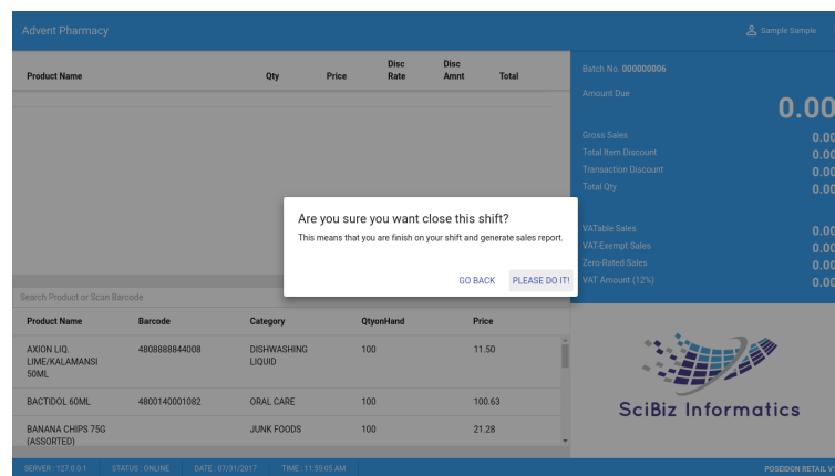
Screenshot 5.8
