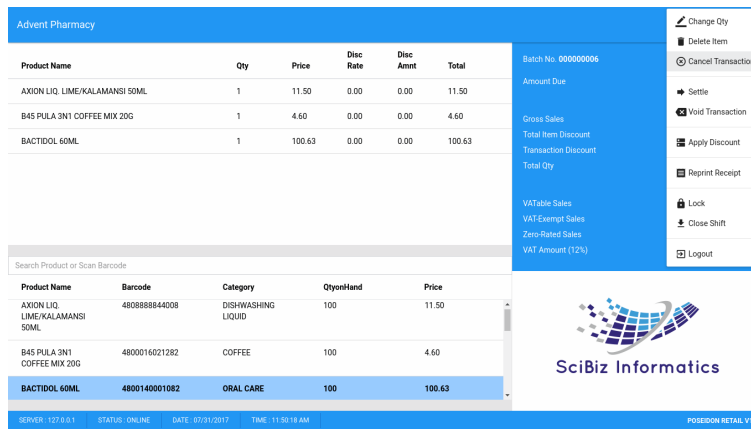
Screenshot 4.3
