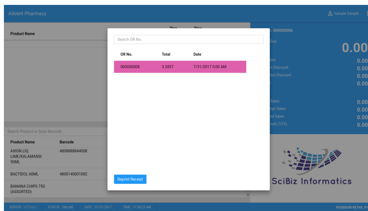
Screenshot 5.3
