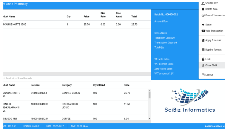
Screenshot 5.7
