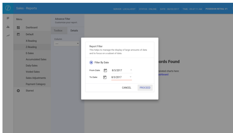
Screenshot 6.5
