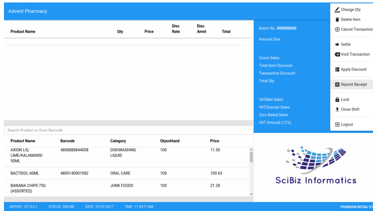
Screenshot 5.2
