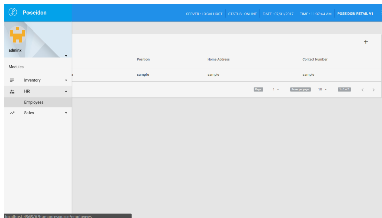
Screenshot 1.2
