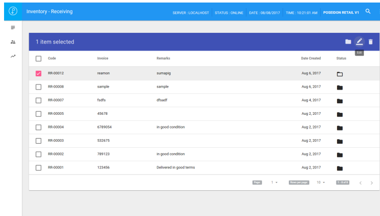
Screenshot 2.9
