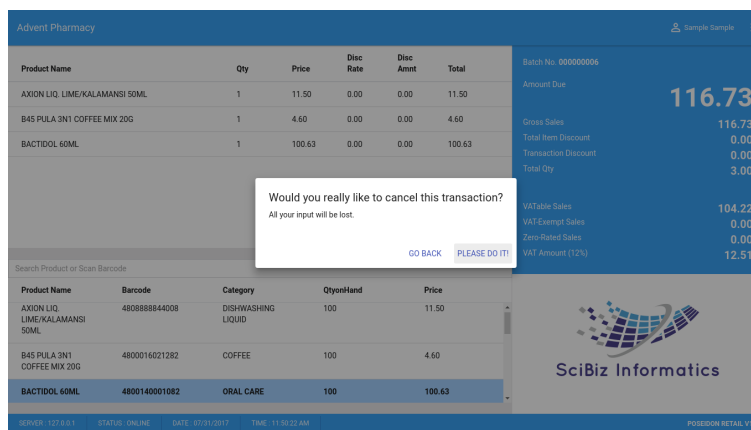
Screenshot 4.4
