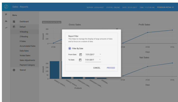
Screenshot 6.3
