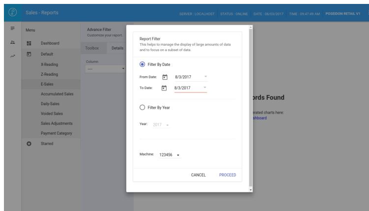
Screenshit 6.6
