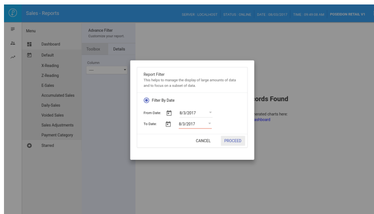
Screenshot 7.0
