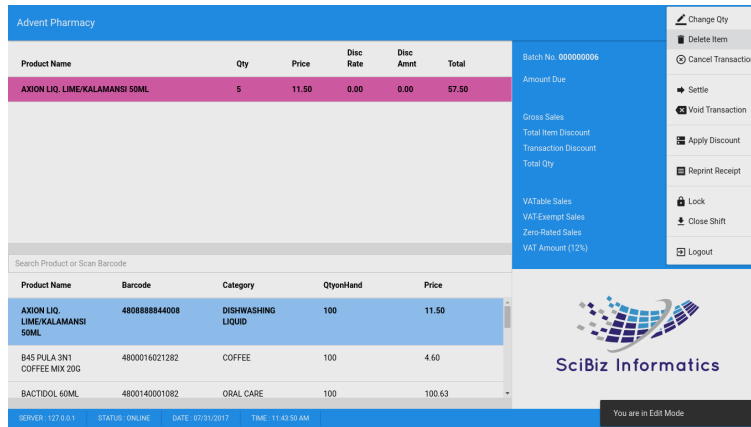
Screenshot 4.1
