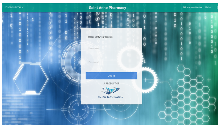
Screenshot 1.0
