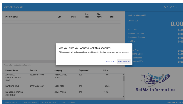
Screenshot 5.5
