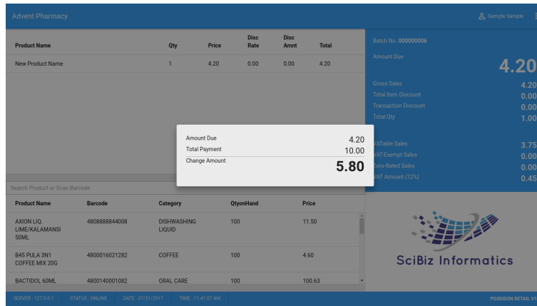
Screenshot 3.9
