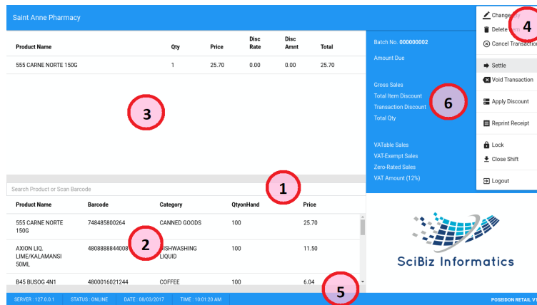
Screenshot 3.4
