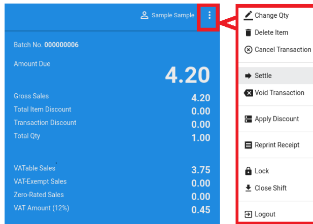
Screenshot 3.7
