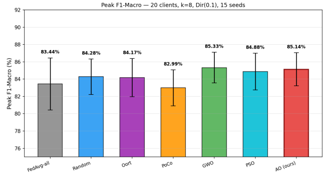
Fig. 1. Peak F1-macro (mean ± std, 15 seeds) for each method.
