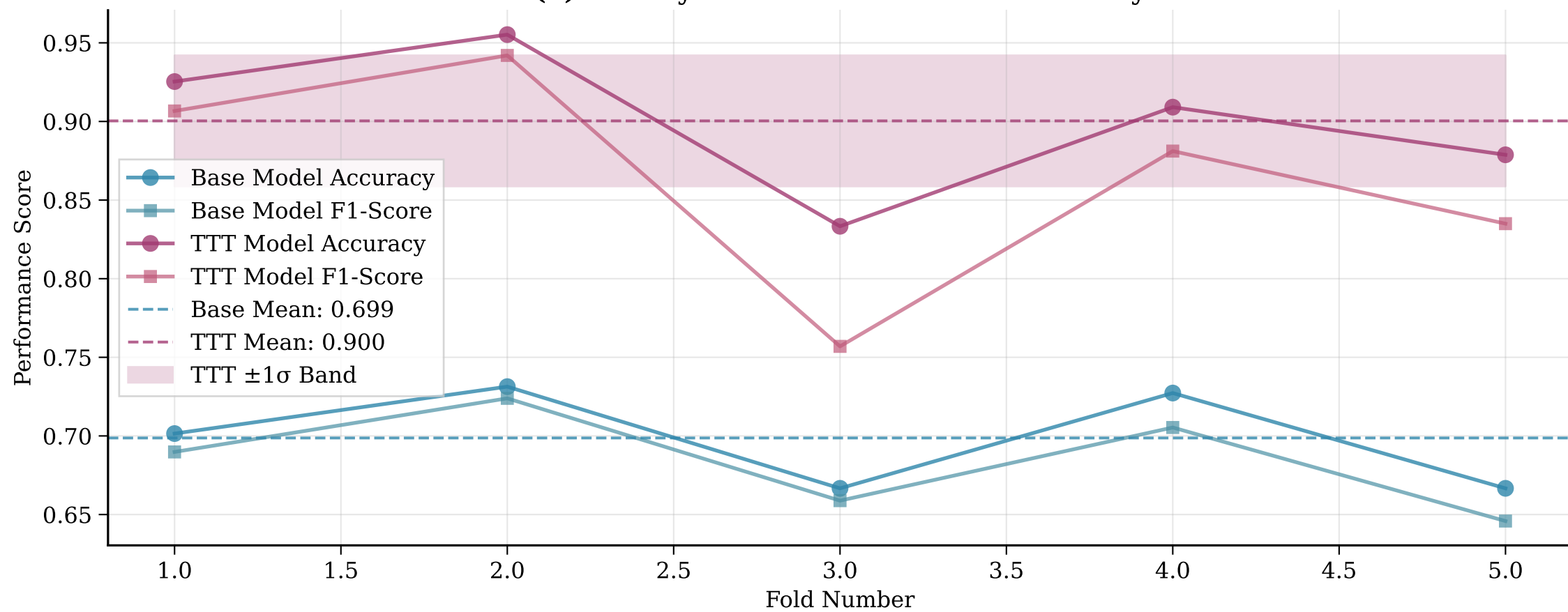
(b) Fold-by-Fold Performance Consistency
