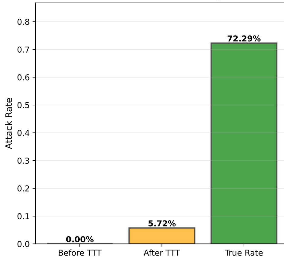
Attack Prediction Rate Comparison
