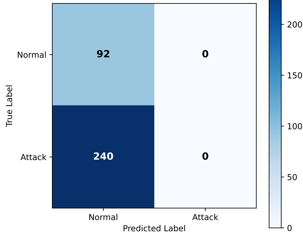
Confusion Matrix: Before TTT
