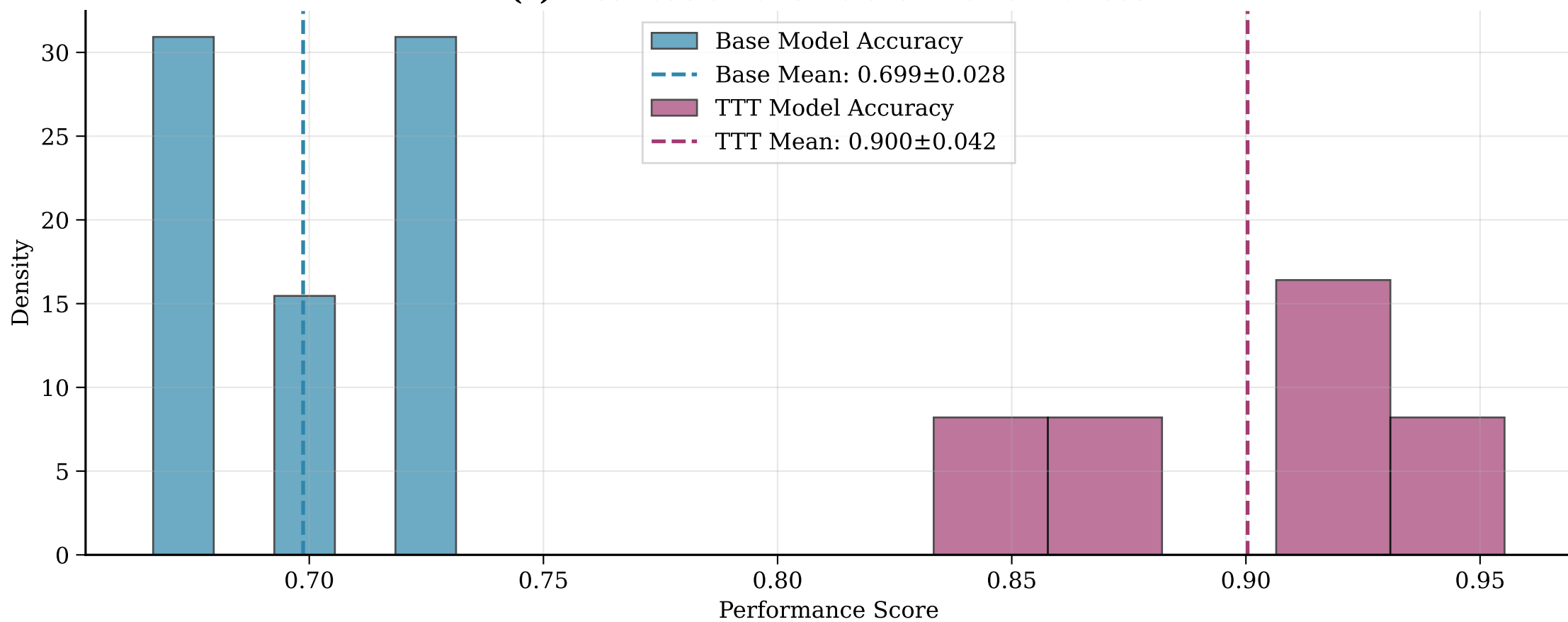
(b) Fold-by-Fold Performance Consistency
