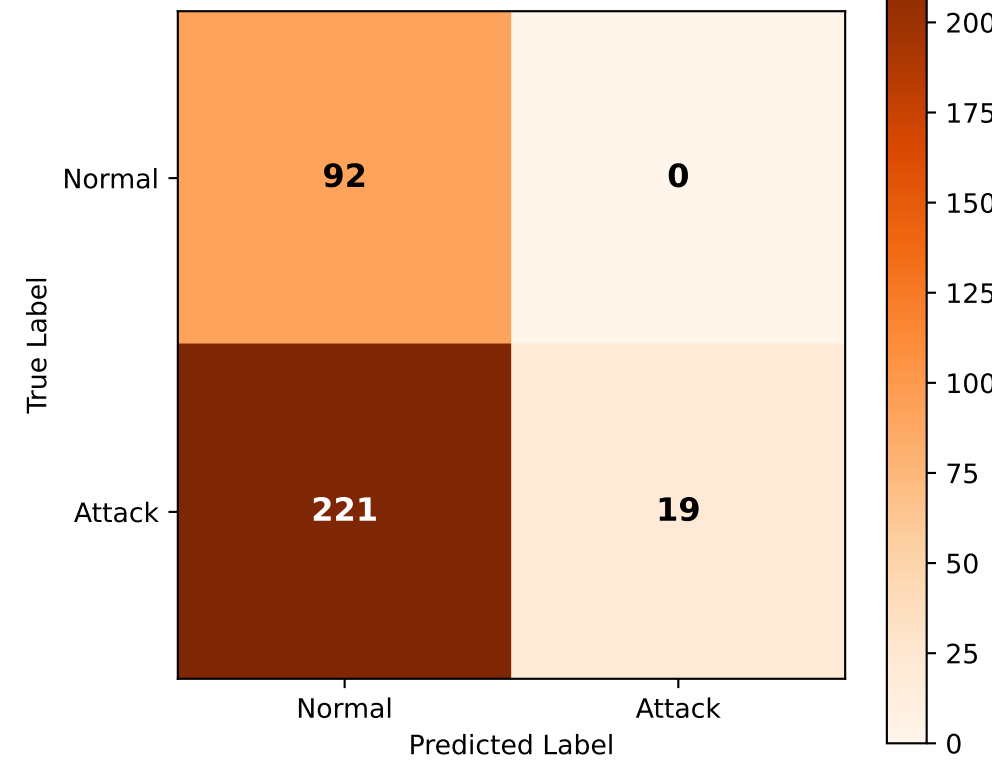
Confusion Matrix: After TTT
