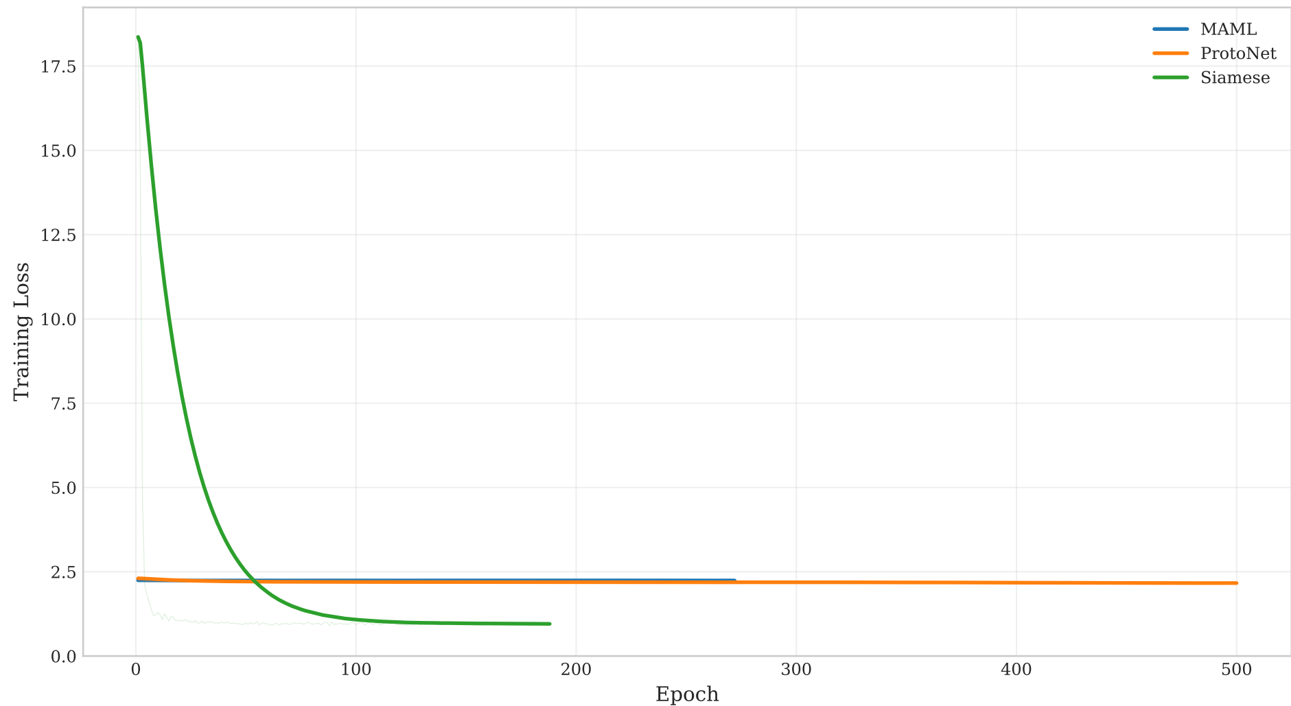
Meta-Learning Training Loss Curves — CHES CTF 2018 (STM32, ARM) (20-shot)
