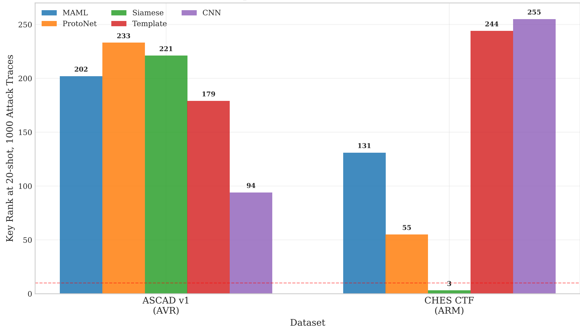
Cross-Dataset Comparison (HW Model, 20-shot, 1000 Traces)
