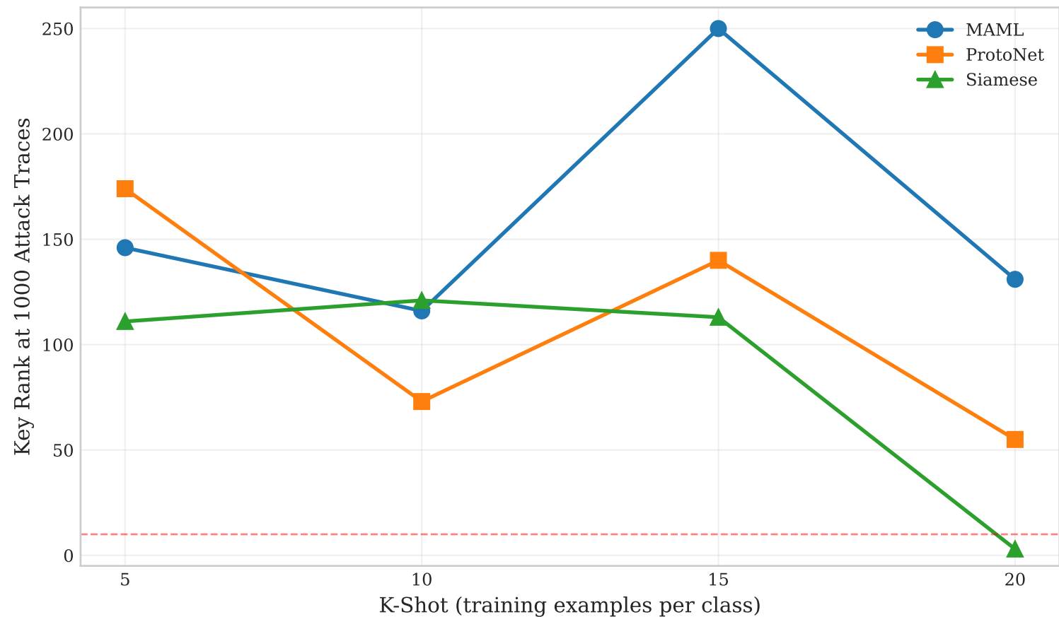
K-Shot Ablation — CHES CTF 2018 (HW Model)
