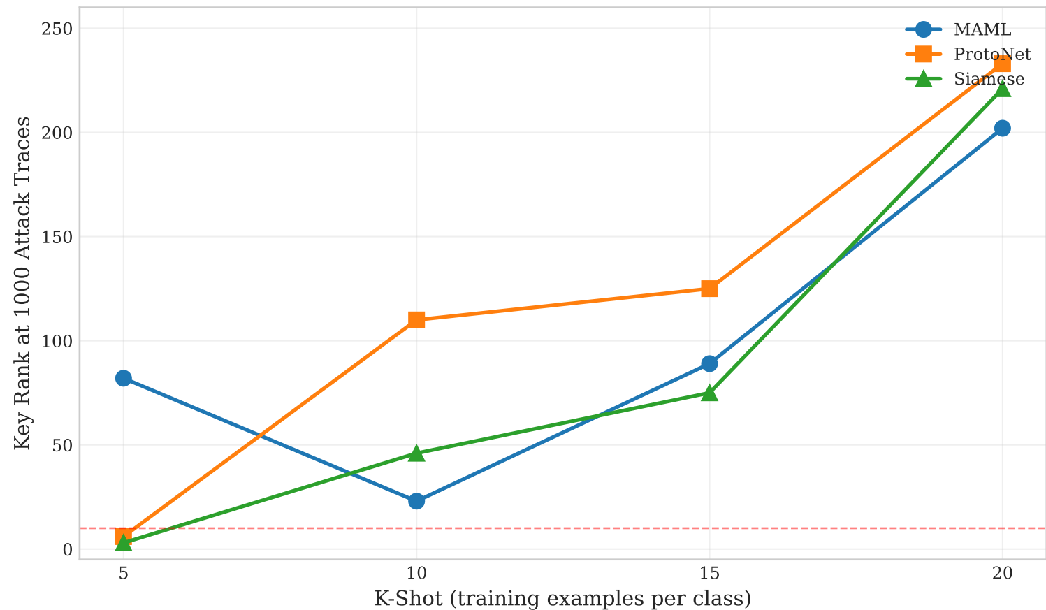
K-Shot Ablation — ASCAD v1 (HW Model)
