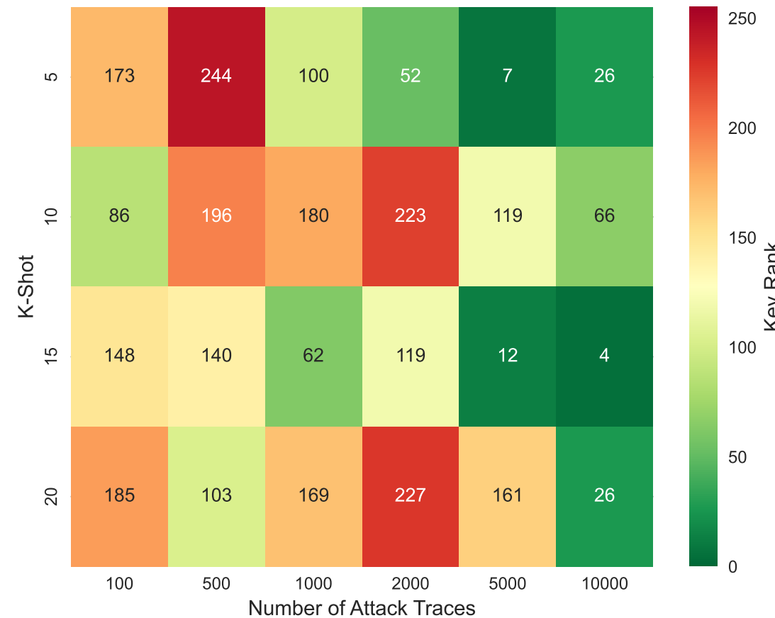
Siamese Performance
