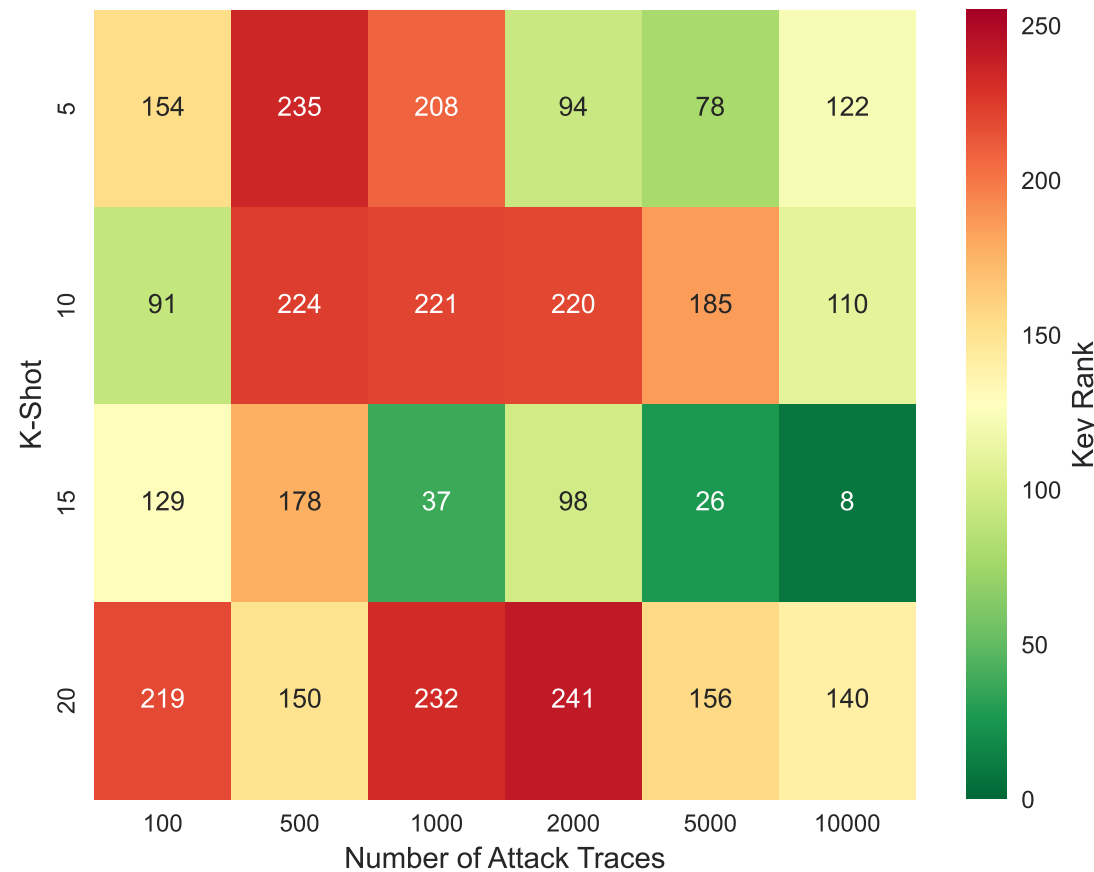
ProtoNet Performance
