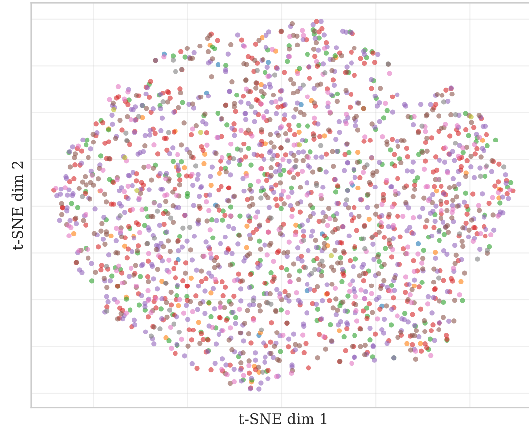
ProtoNet
