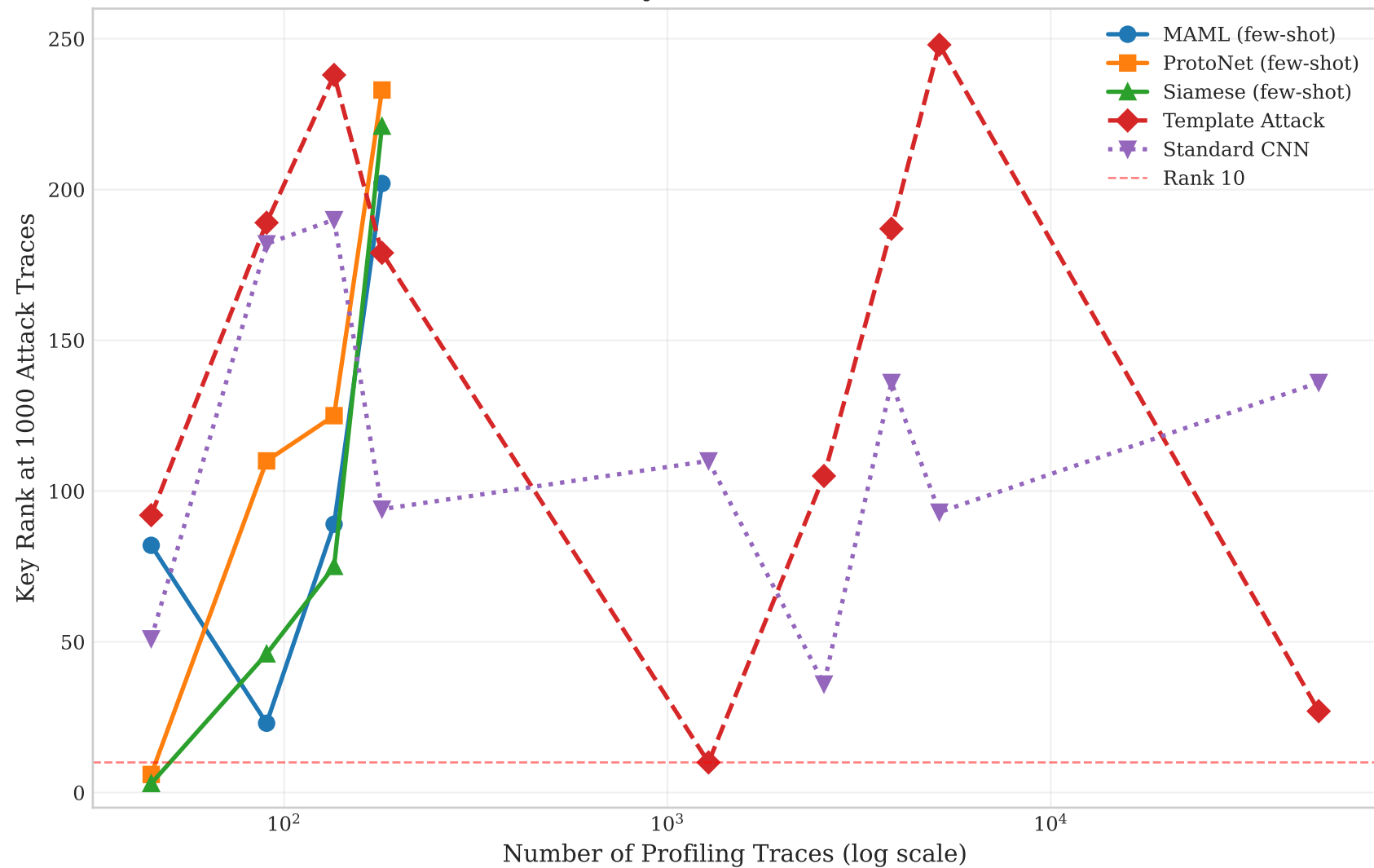
Data Efficiency — ASCAD v1 (HW Model)
