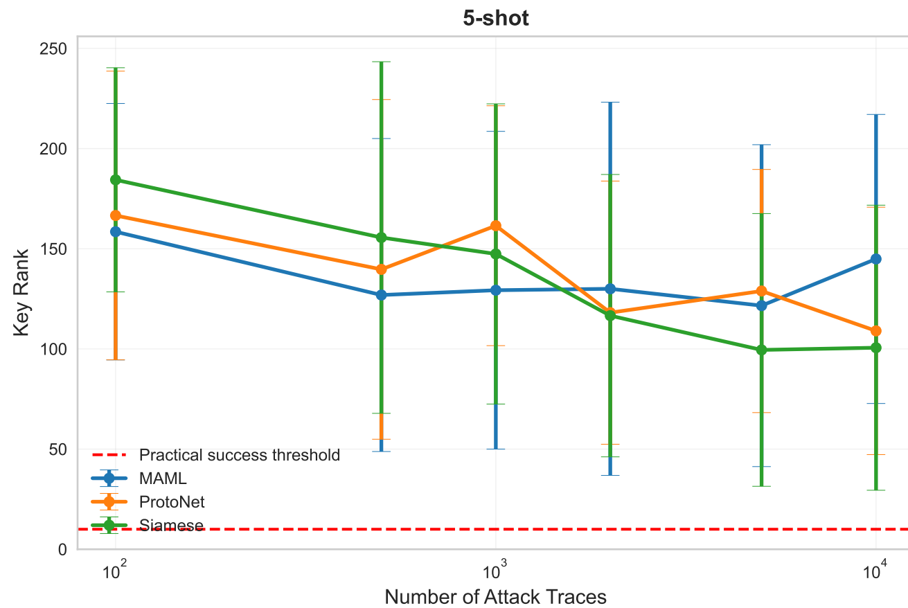
Key Rank vs. Number of Attack Traces for Different Few-Shot Settings (with Minimal Variance Sampling)
