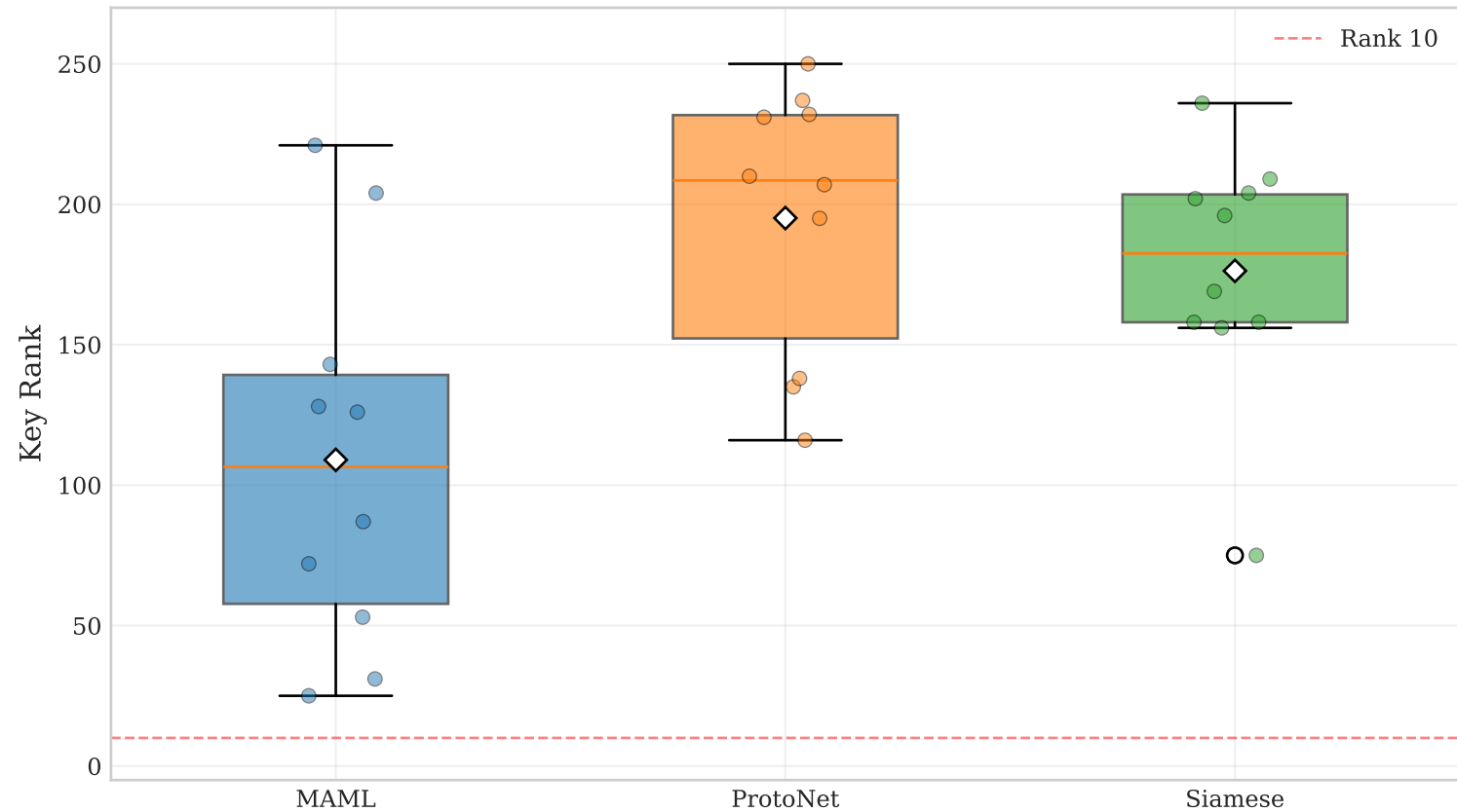
Key Rank Distribution — ASCAD v1 (ID) (20-shot, 1000 traces, 10 runs)
