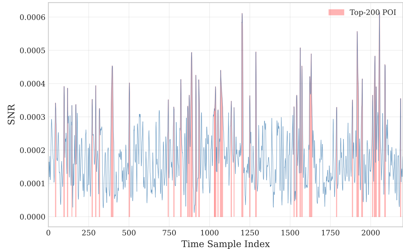
CHES CTF 2018 (STM32, 32-bit ARM)
