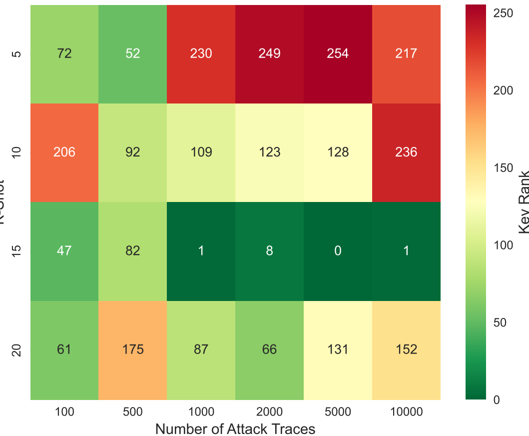
MAML Performance
