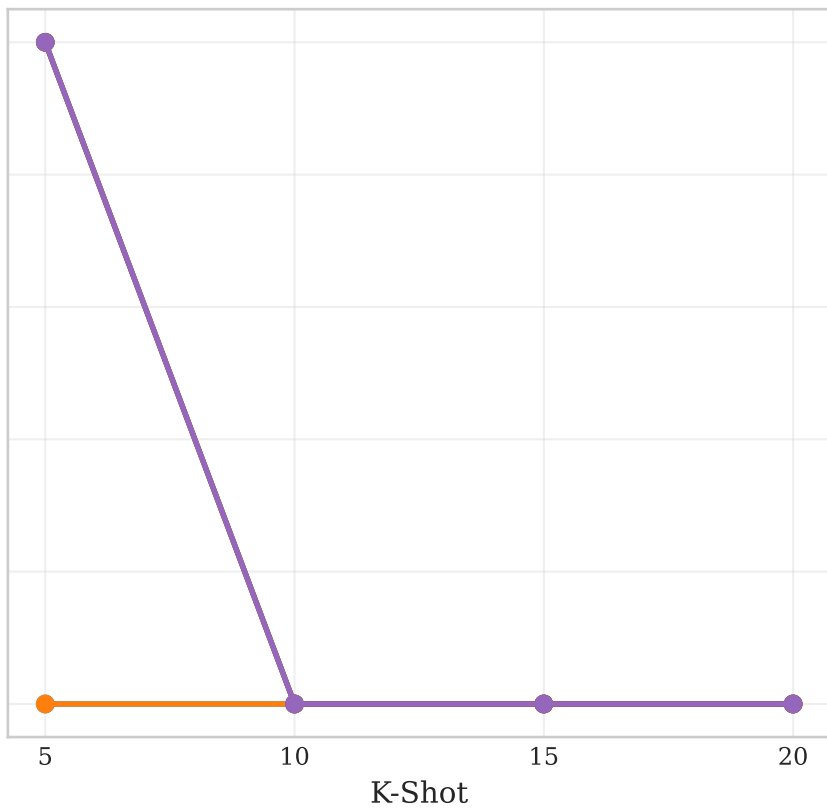
ProtoNet
