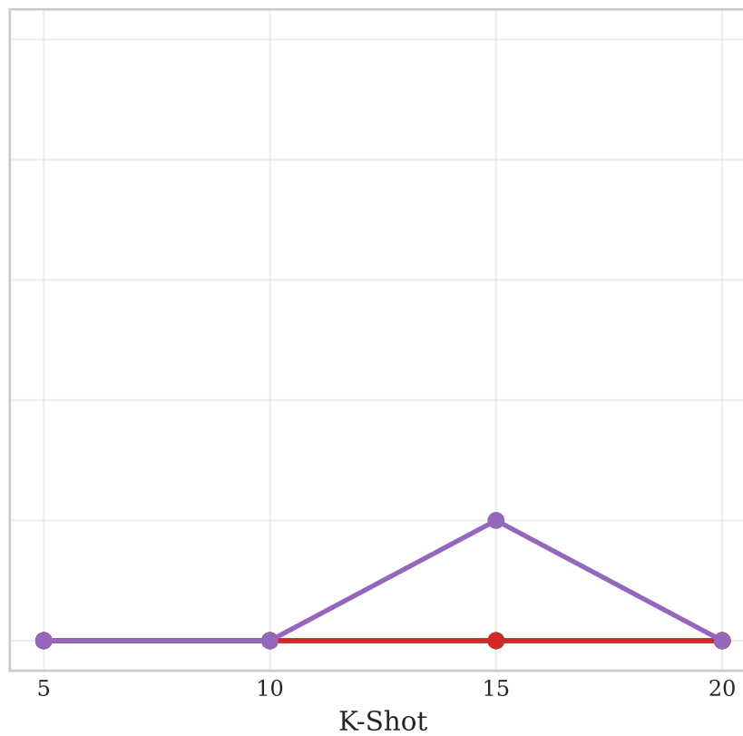
ProtoNet
