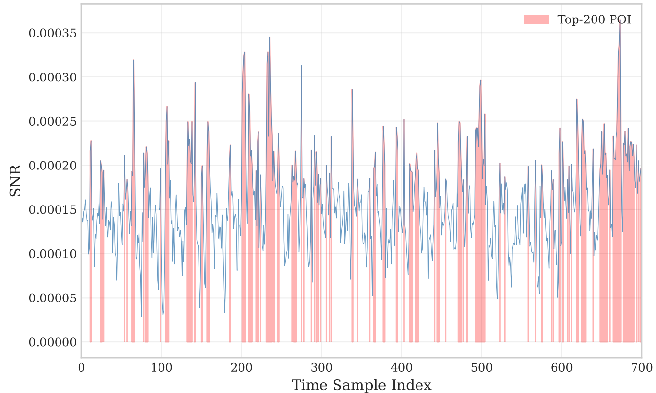
ASCAD v1 (ATMega8515, 8-bit AVR)
