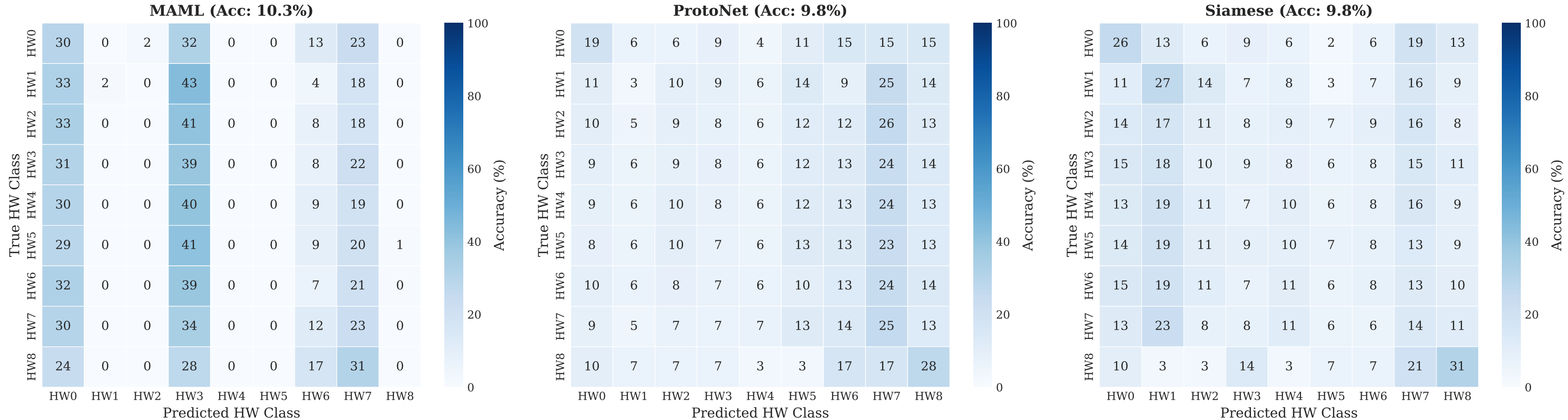
HW Class Confusion Matrix — CHES CTF 2018 (STM32, ARM) (20-shot, validation set, row-normalized %)
