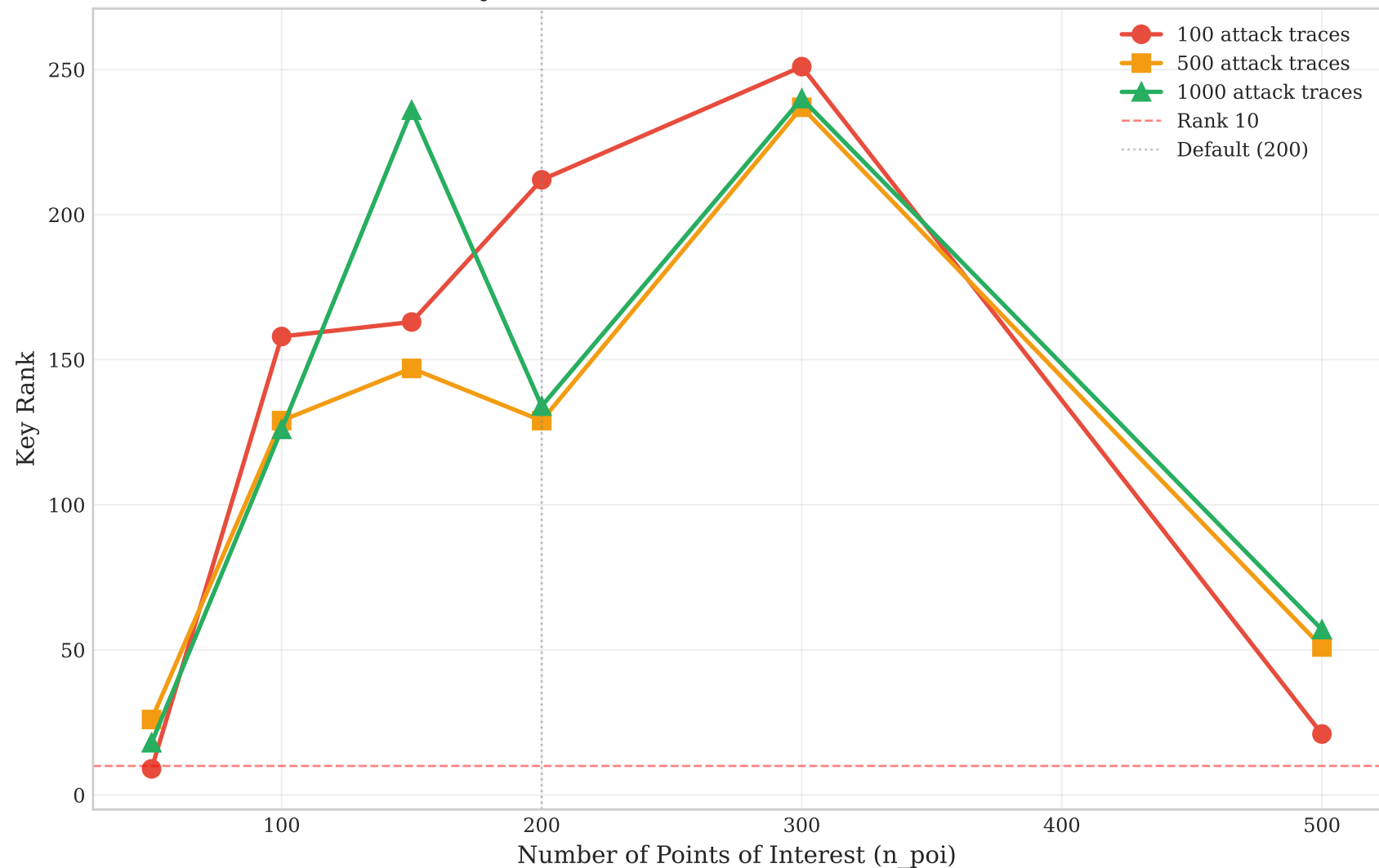
POI Ablation Study — Siamese 20-shot, CHES CTF 2018 (STM32, ARM)
