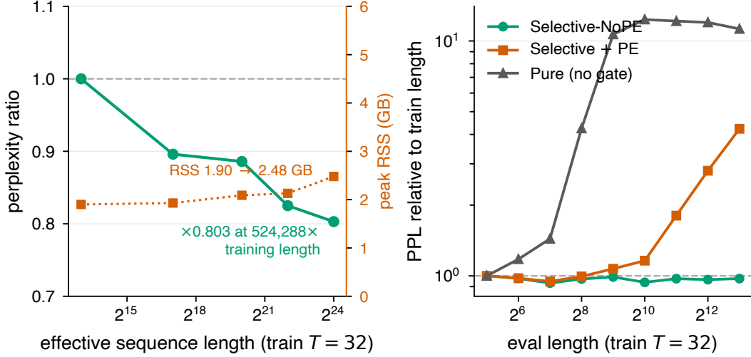
Figure 7: Length, re-anchored. Left : perplexity ratio and peak RSS against effective sequence length — \times 0.803 at 524,288\times the training length, improving monotonically, at 1.90→2.48 GB. Right : the control. Position-free Selective holds \times 0.973 to 256\times ; the same architecture with a positional encoding degrades to \times 4.23 and the ungated arm to \times 11.25 . Sources: results/scale_to_a_million.json , results/length_extrap_v2_extreme.json .
