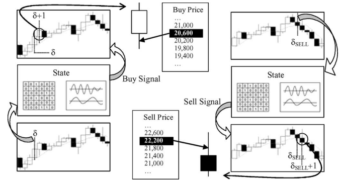
Fig. 2. Sample episode.
