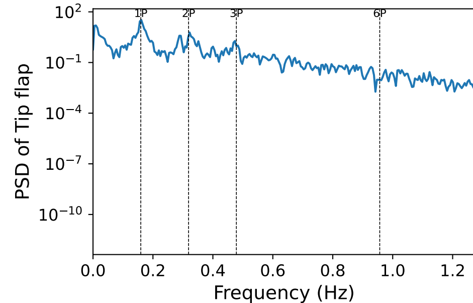
Q1 — PSDs, V0=18 m/s, omega_mean=1.00 rad/s
