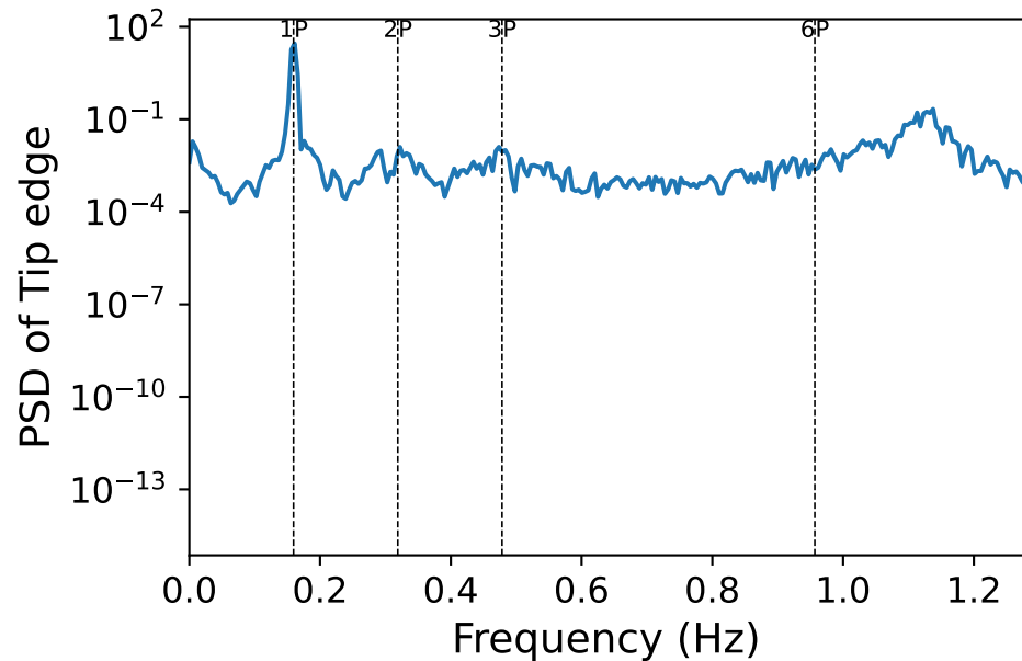
Q1 — PSDs, V0=18 m/s, omega_mean=1.00 rad/s
