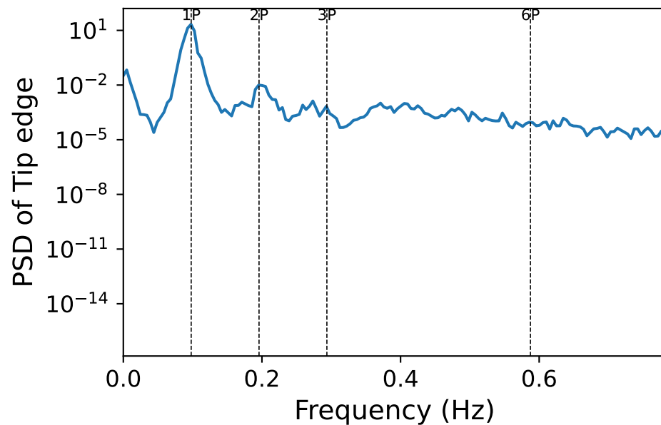
Q1 — PSDs, V0=7 m/s, omega_mean=0.62 rad/s
