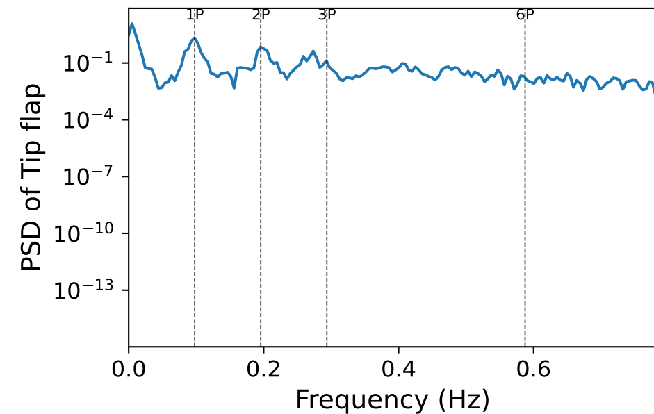
Q1 — PSDs, V0=7 m/s, omega_mean=0.62 rad/s
