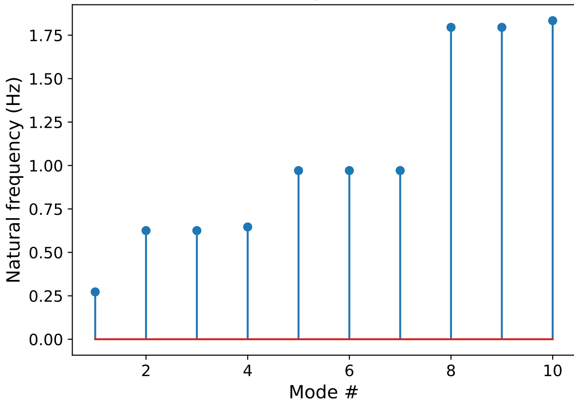
Q3 — 11-DOF natural frequencies (azimuth removed)
