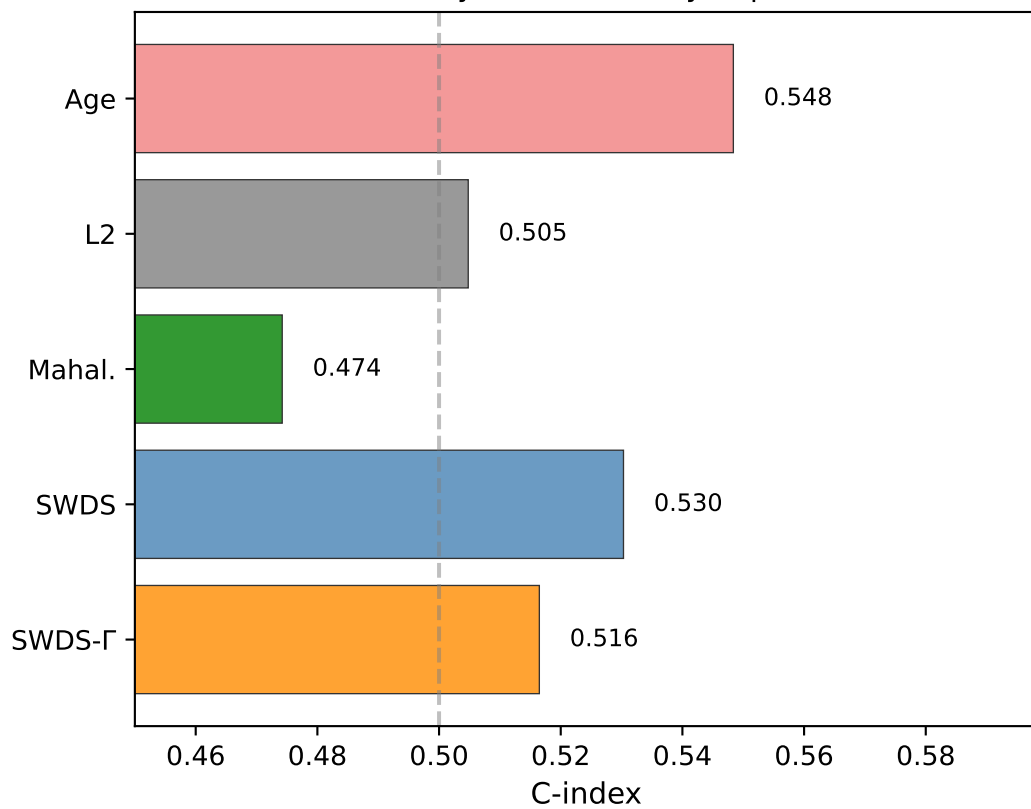
(c) Discrimination: synthetic stability-dependent outcome
