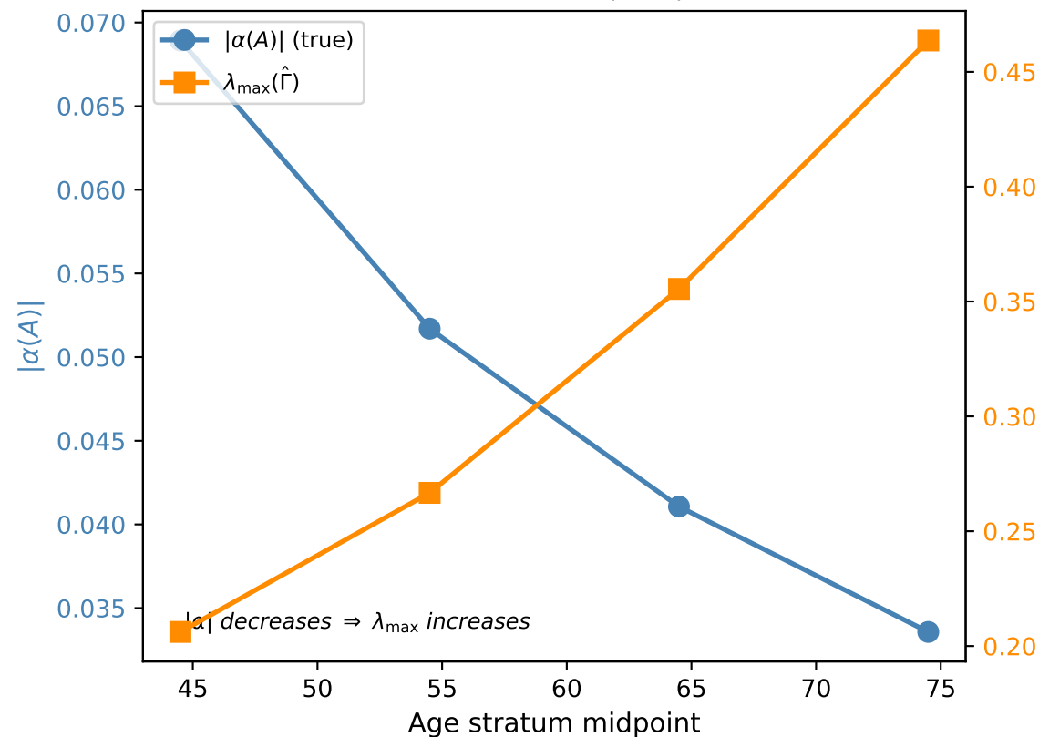
(c) Discrimination: synthetic stability-dependent outcome
