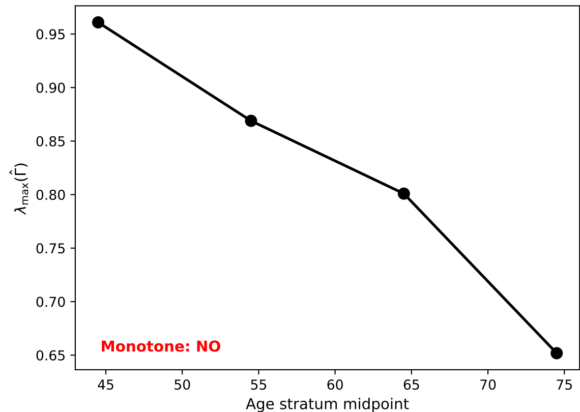
(c) SWDS- \Gamma distribution by age stratum
