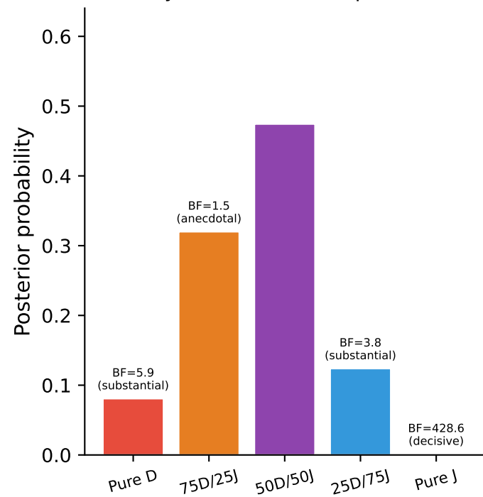
(a) Bayesian model comparison
