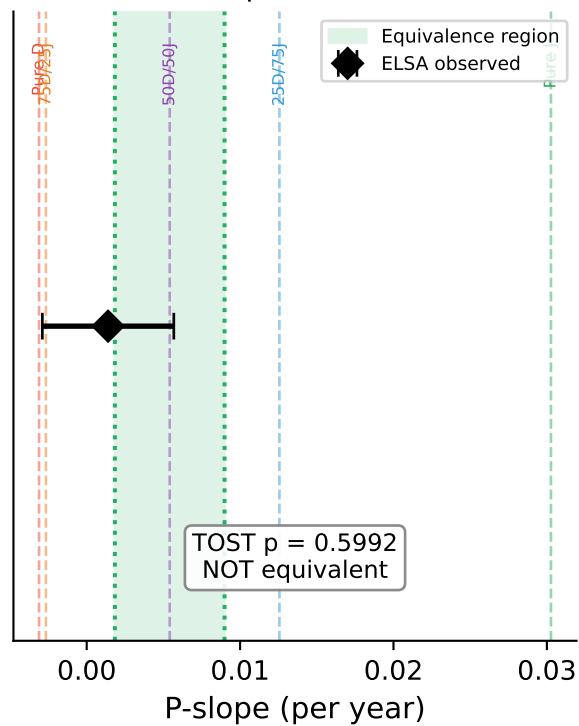
(b) TOST equivalence test
