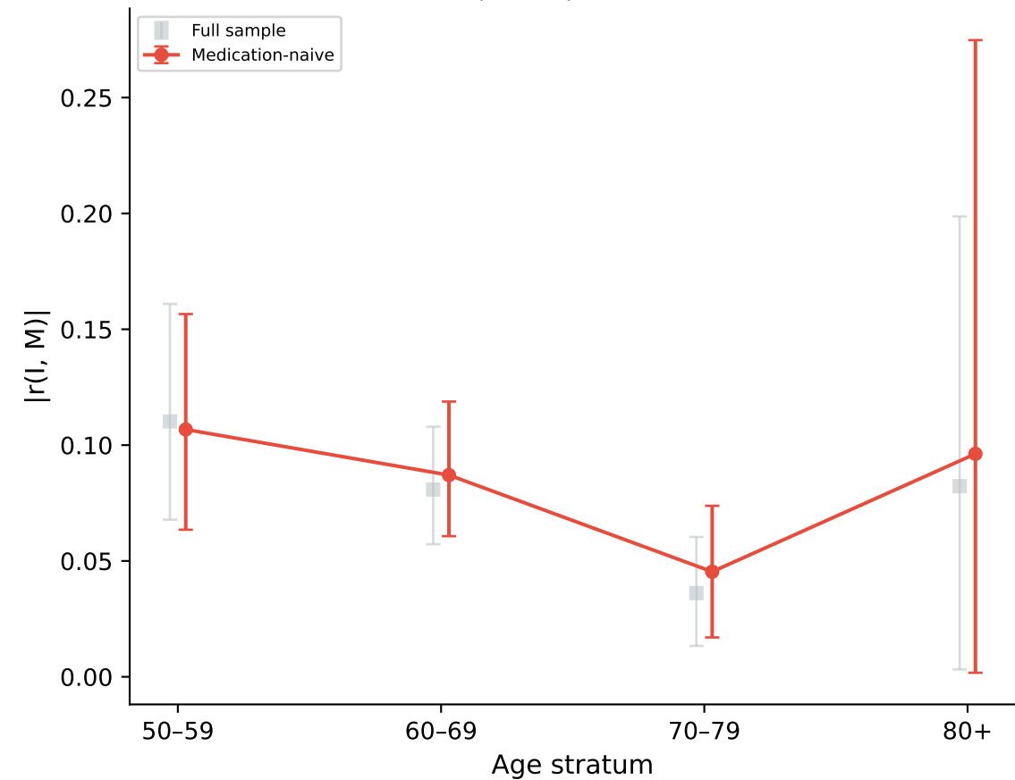
|r(I, M)| vs age
