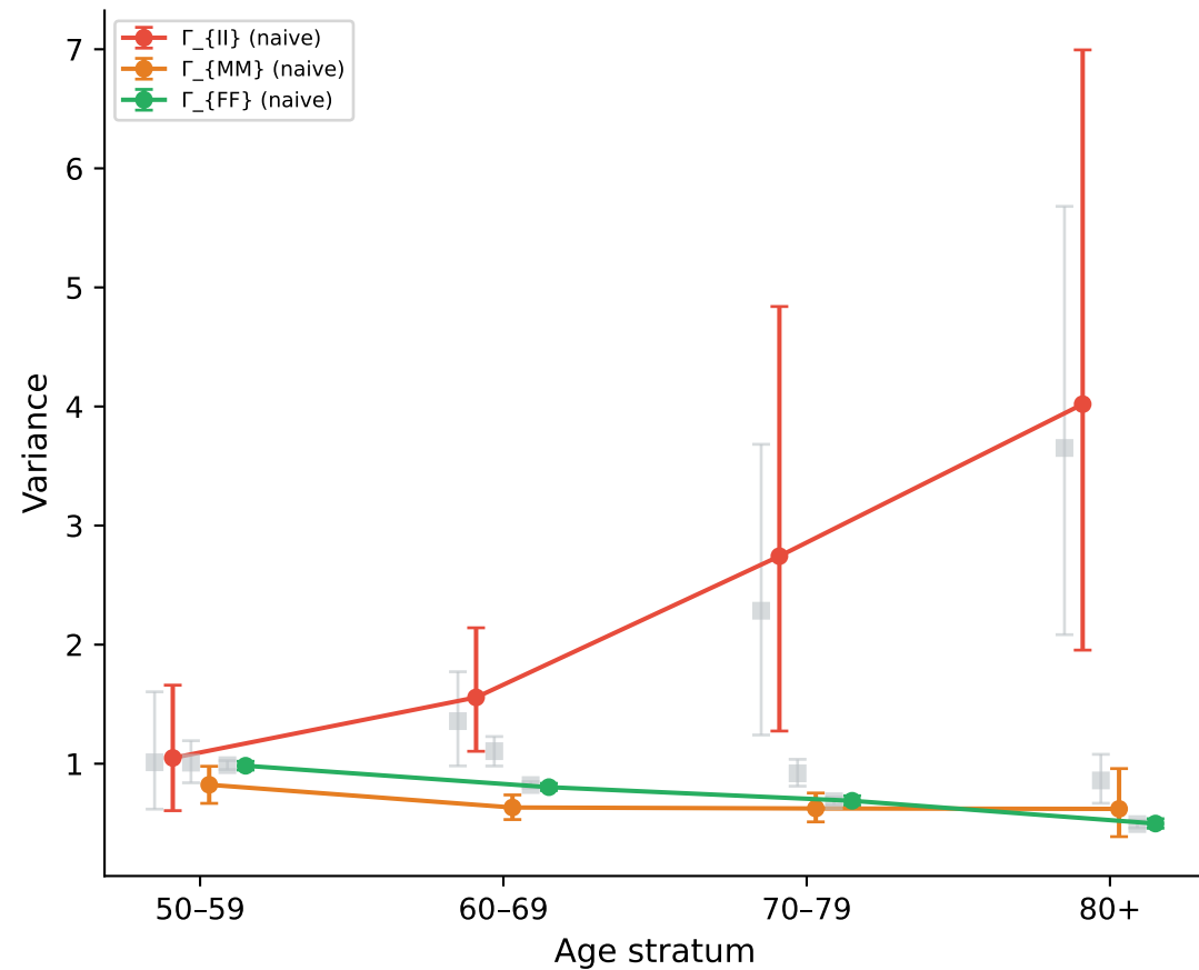
Individual axis variances
