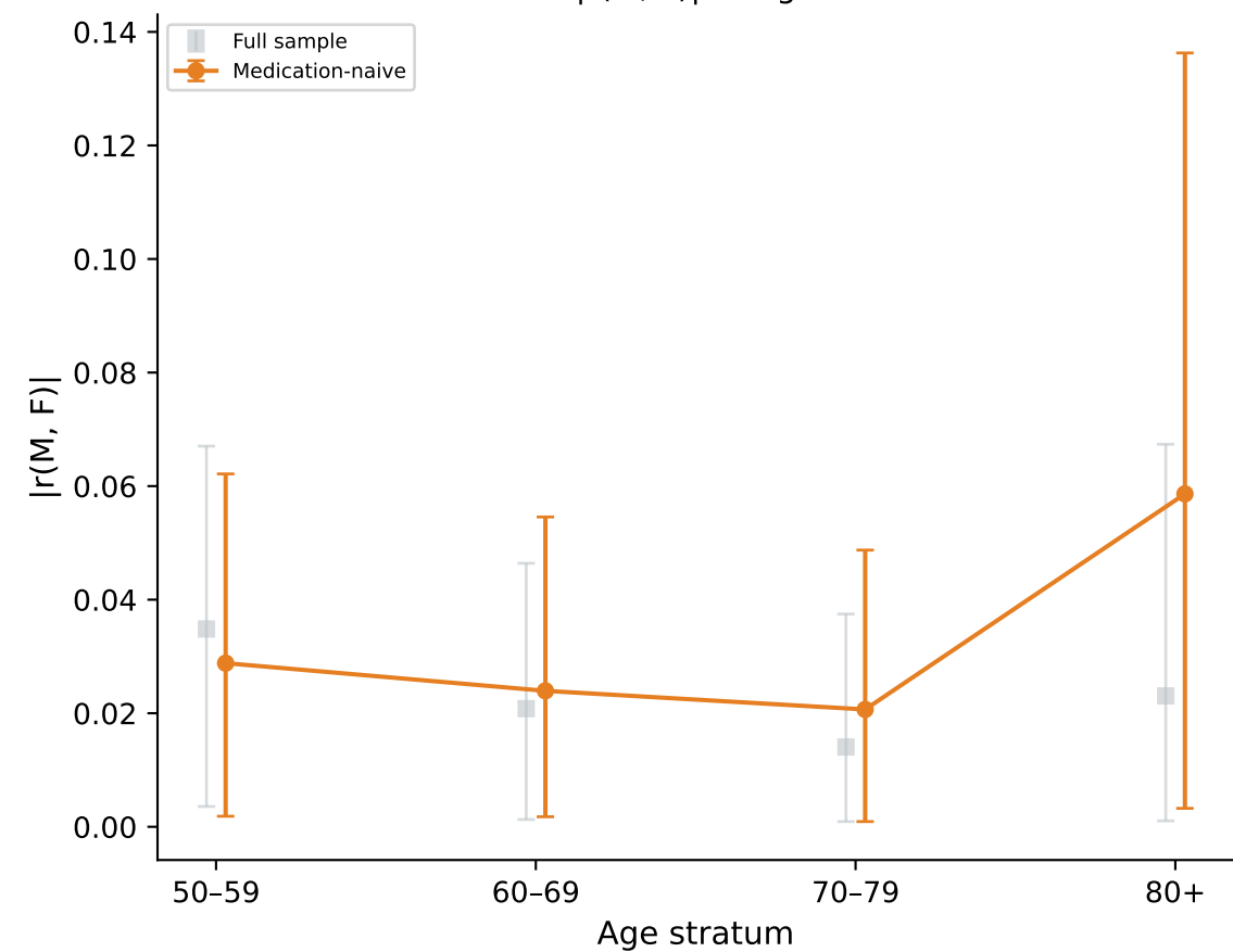
|r(M, F)| vs age
