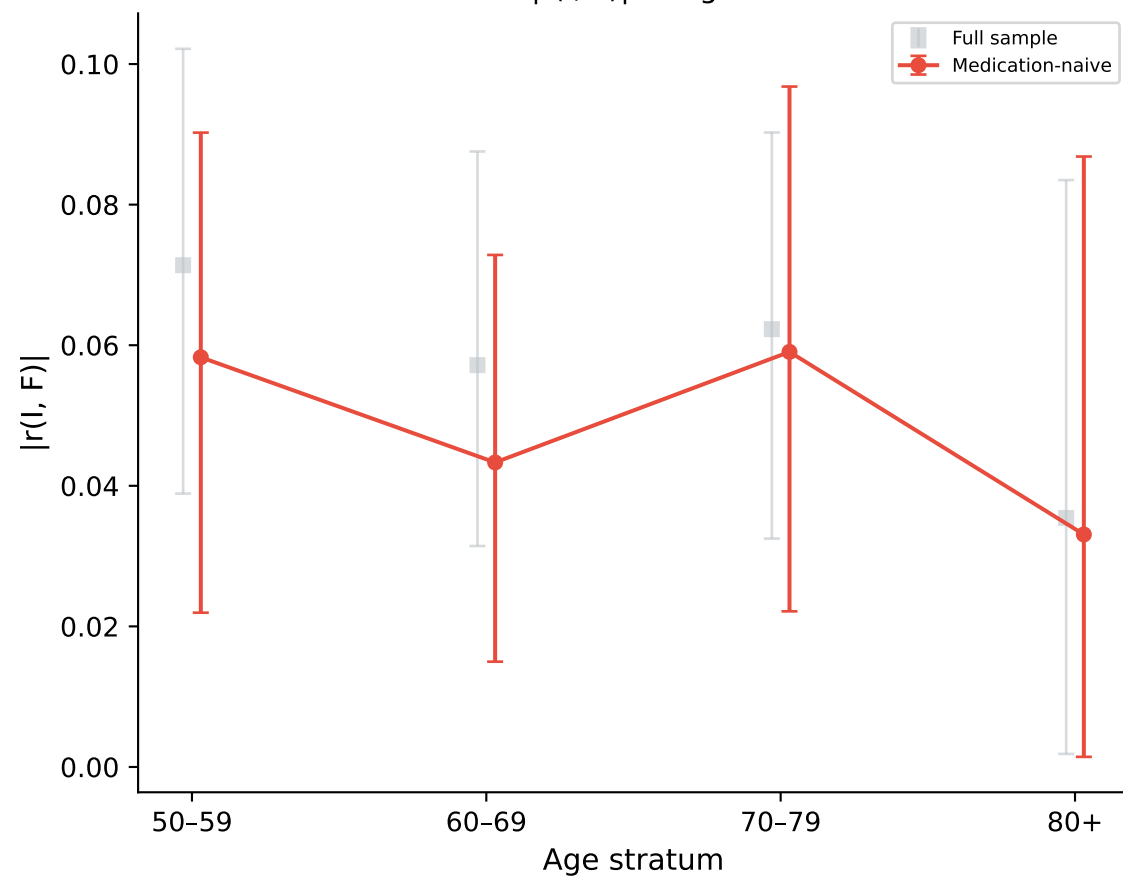
|r(I, F)| vs age
