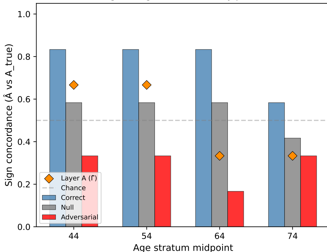
(a) Off-diagonal sign concordance by prior condition
