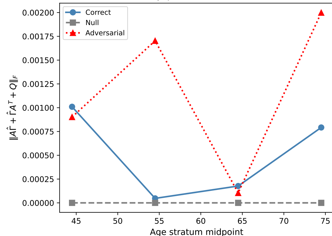
(b) Lyapunov residual norm
