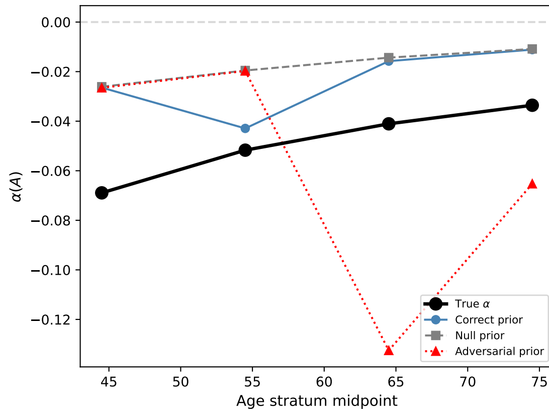
(c) \hat{\alpha} by prior condition vs true \alpha
