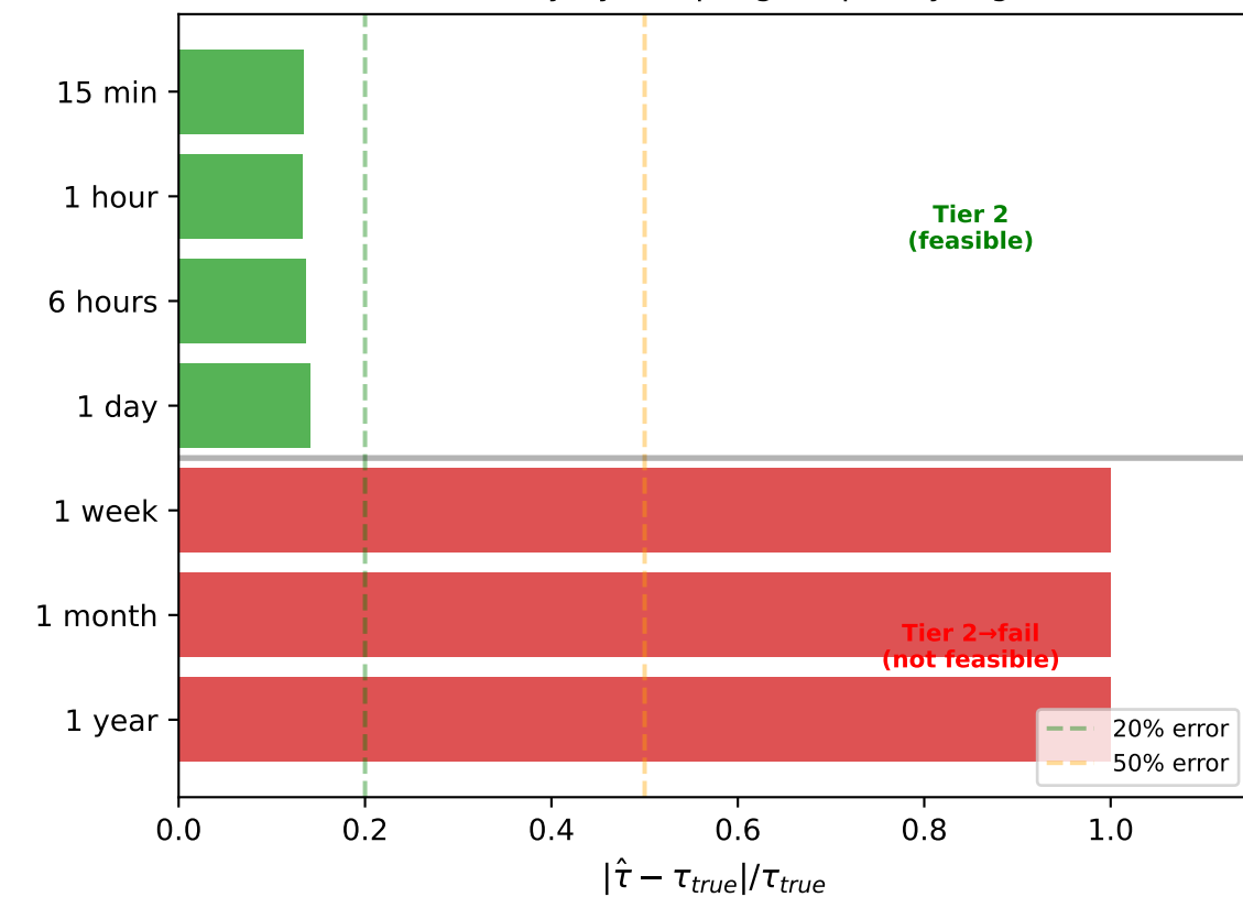
(c) \tau_l recovery by sampling frequency (age 55)
