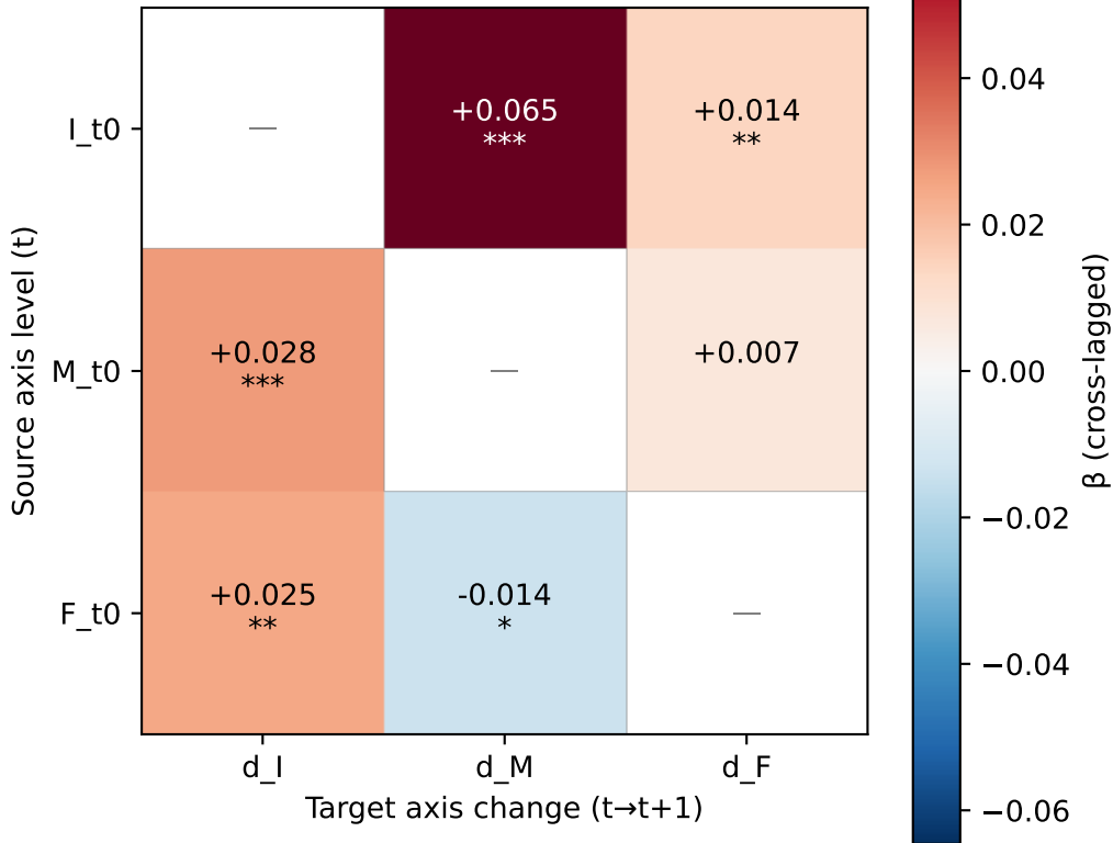
ELSA 3-axis cross-lagged \beta (full sample)
