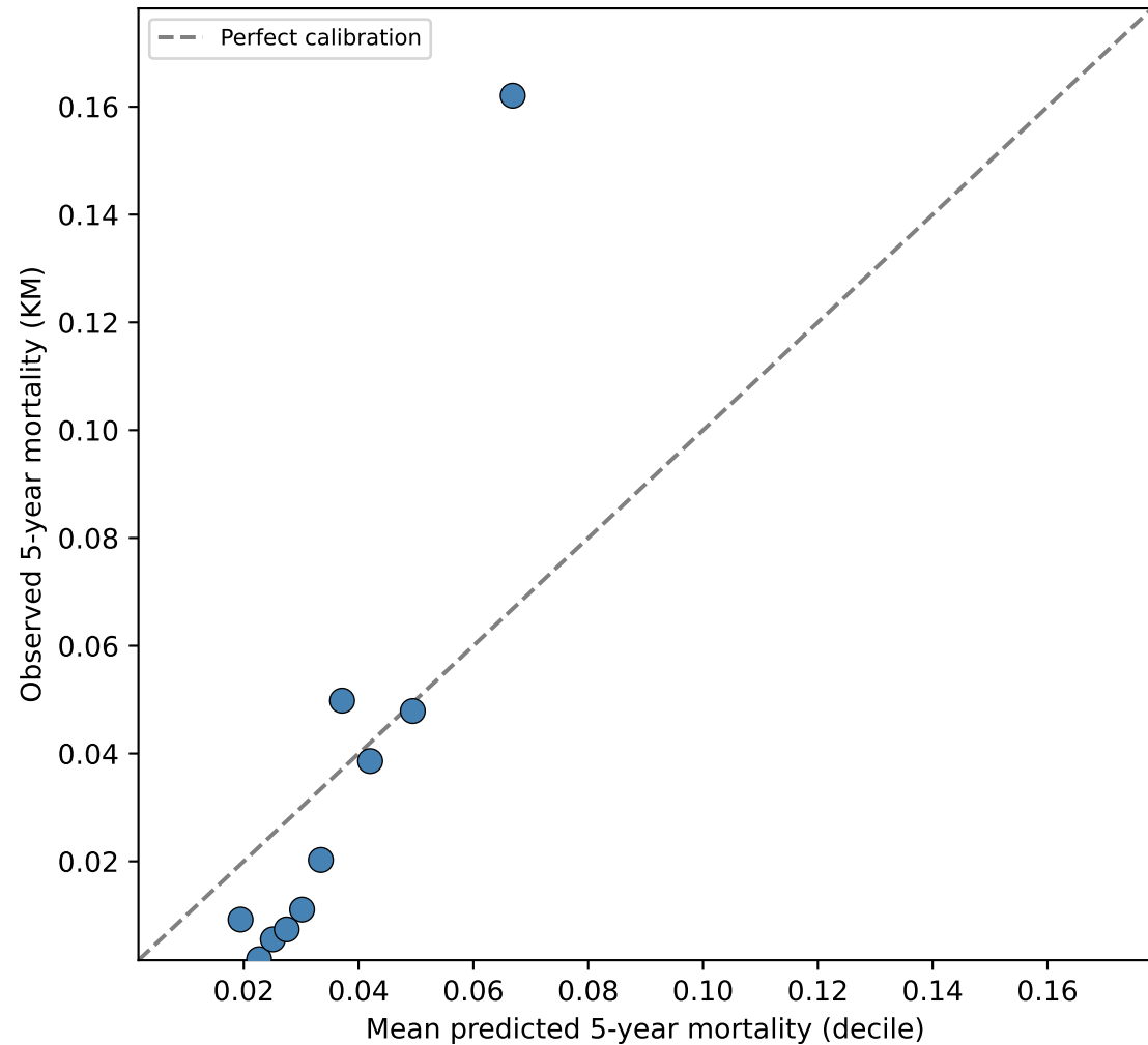
Calibration: M5 HL \chi^2=121.6 , p=0.000
