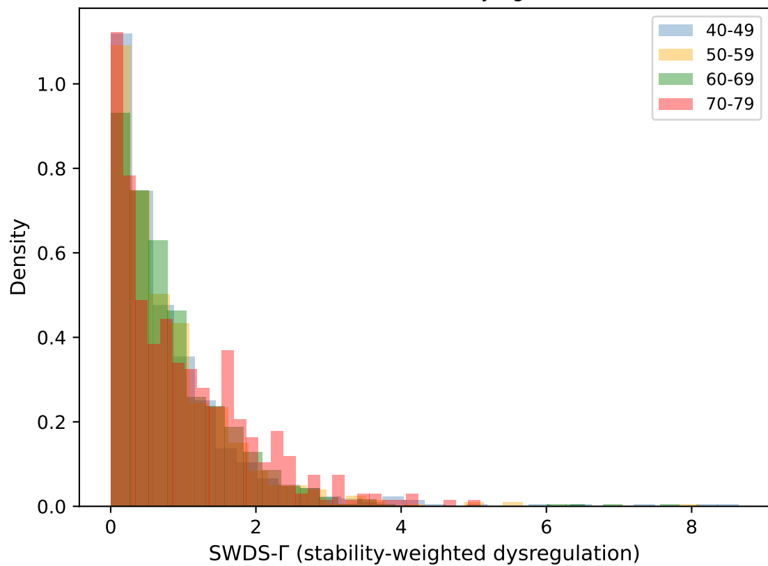
(c) SWDS- \Gamma distribution by age stratum
