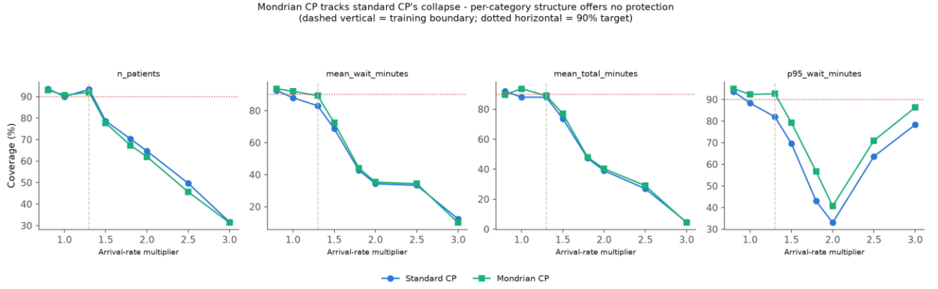
Fig. 6. Standard vs. Mondrian CP coverage across the severity sweep, all four targets. Mondrian CP tracks standard CP's collapse - per-category structure gives no protection outside its own calibrated support.
