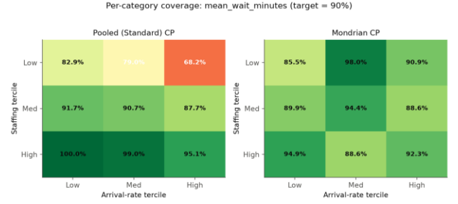
Fig. 3. Department A per-category coverage for mean_wait_minutes: pooled (left) vs. Mondrian (right) calibration across the full 3 \times 3 staffing \times arrival-rate grid.
