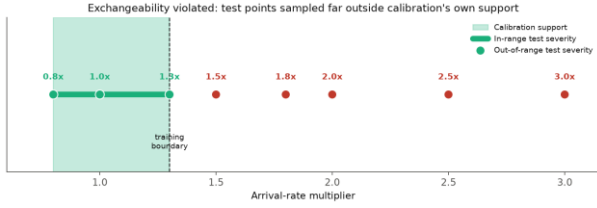
Fig. 2. Calibration support versus test severities used in the exchangeability stress test (Section V-E); the same staffing \times arrival-rate binning is used throughout.
