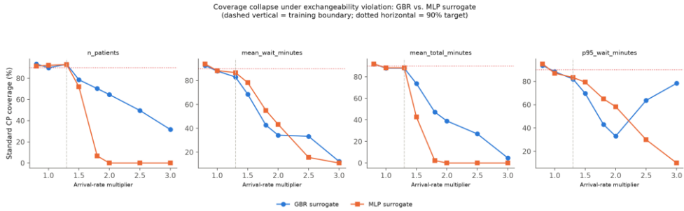
Fig 6.1: Standard conformal prediction coverage vs. arrival-rate severity, gradient-boosting vs. MLP surrogate, all four targets.
