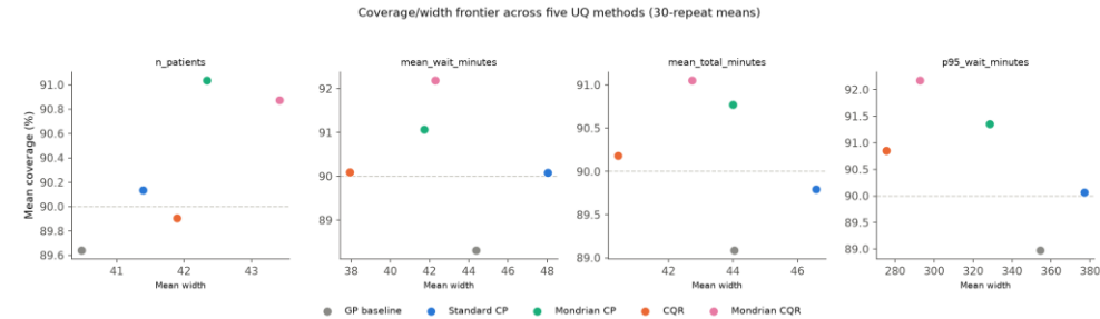
Fig. 6.1. Coverage/width frontier across all five UQ methods, 30-repeat means, per target.
