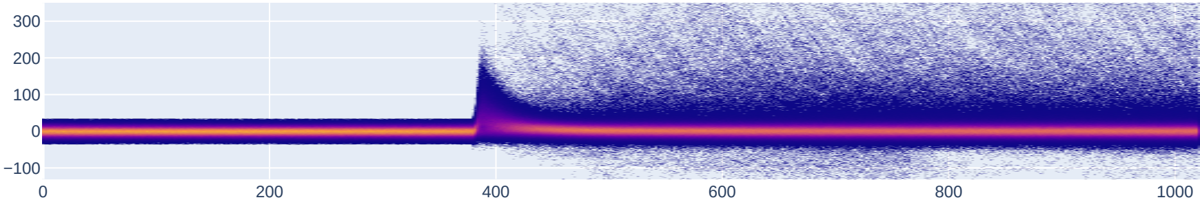
Persistence – Baseline adcs cut: 15545 wfs
