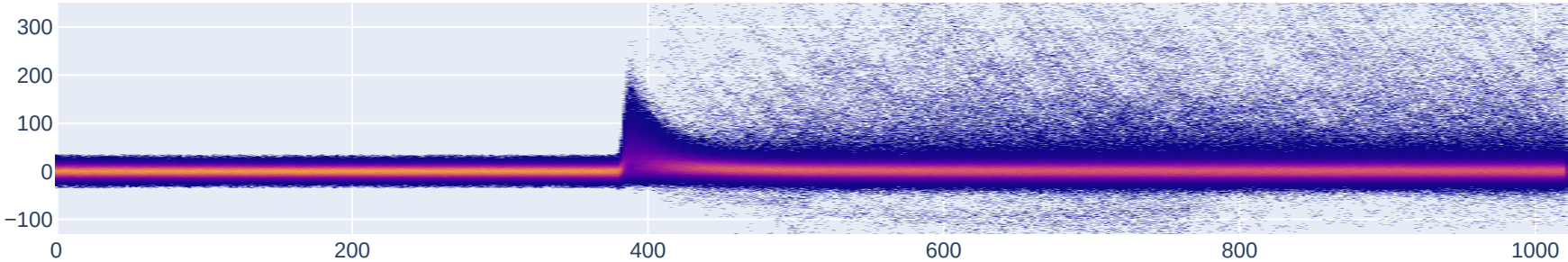
Persistence – Baseline std cut: 8703 wfs
