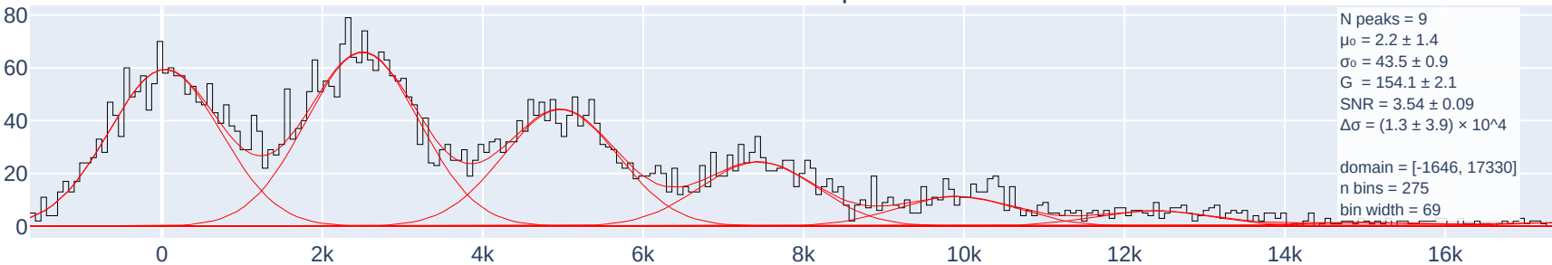
Calibration plot
