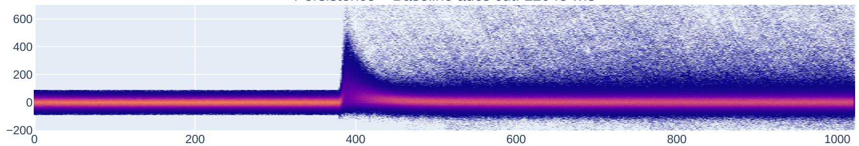
Persistence – Baseline adcs cut: 12043 wfs
