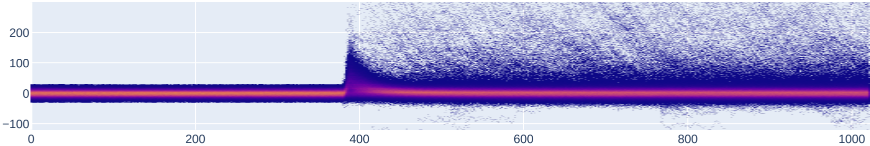
Persistence – Baseline adcs cut: 13639 wfs
