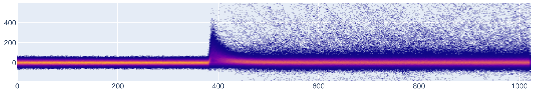
Persistence – Baseline std cut: 8391 wfs
