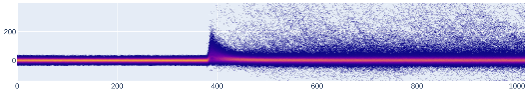
Persistence – Baseline std cut: 9578 wfs
