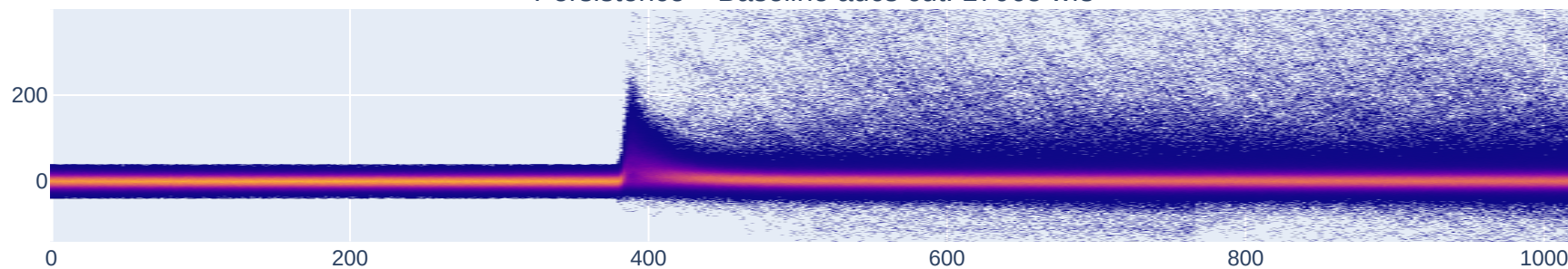
Persistence – Baseline adcs cut: 17065 wfs
