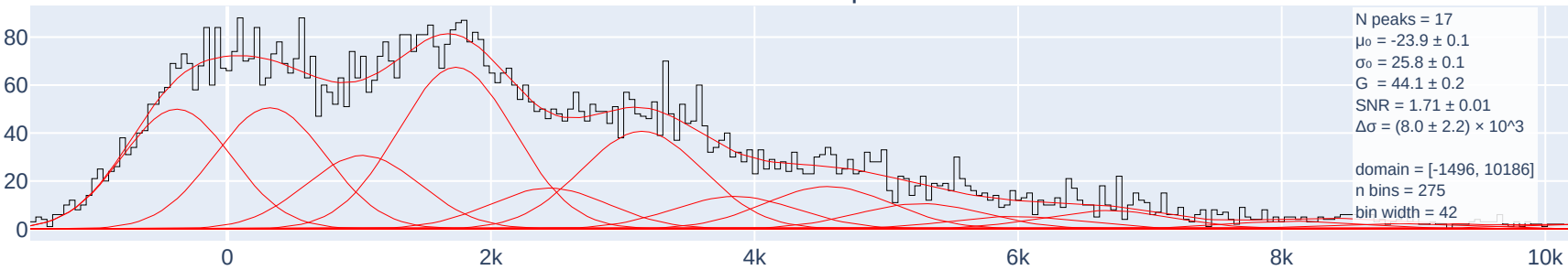
Calibration plot
