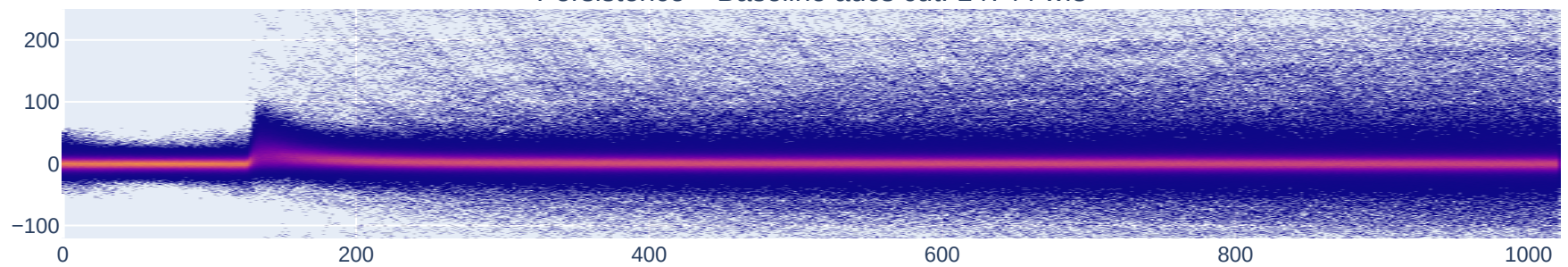
Persistence – Baseline adcs cut: 14744 wfs
