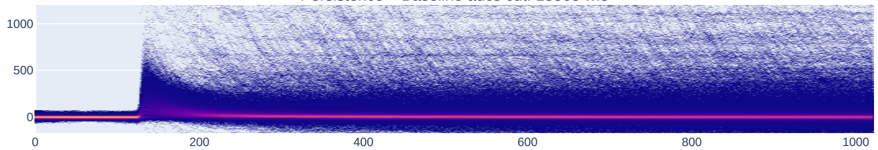
Persistence – Baseline adcs cut: 13363 wfs
