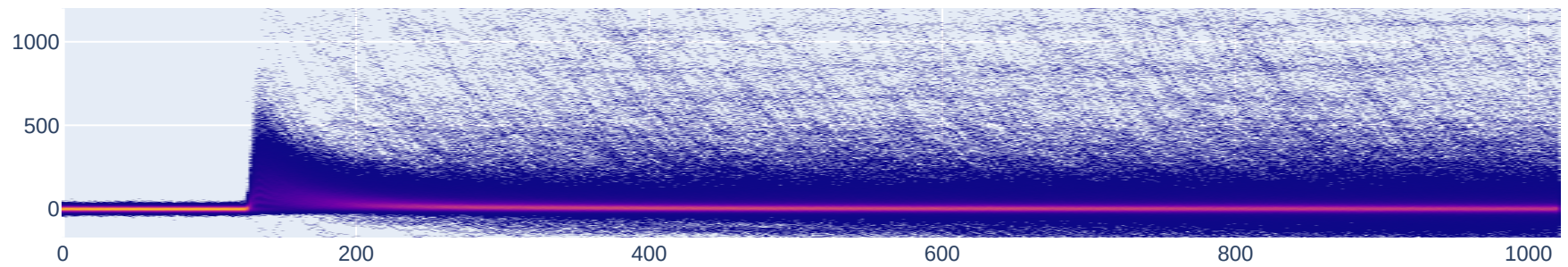
Persistence – Baseline std cut: 8696 wfs
