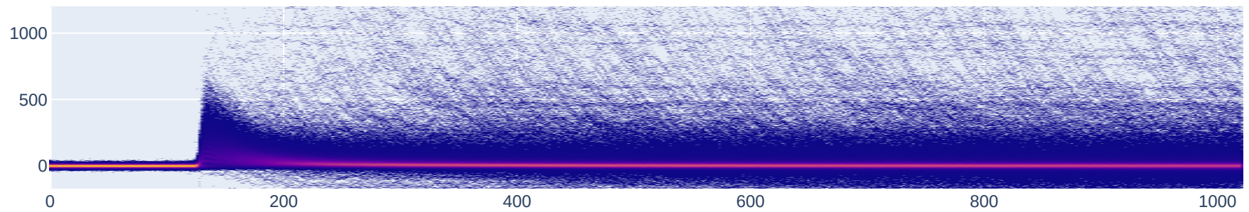
Persistence – Baseline std cut: 9222 wfs
