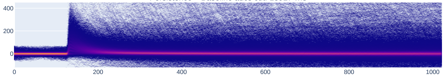
Persistence – Baseline adcs cut: 13917 wfs
