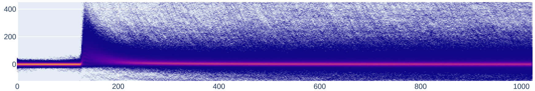
Persistence – Baseline std cut: 12773 wfs
