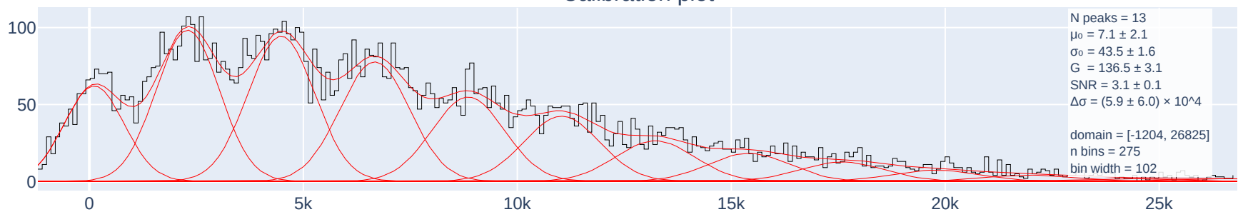
Calibration plot
