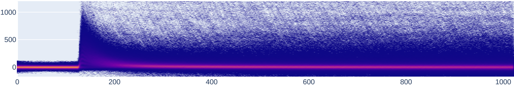
Persistence – Baseline adcs cut: 13301 wfs
