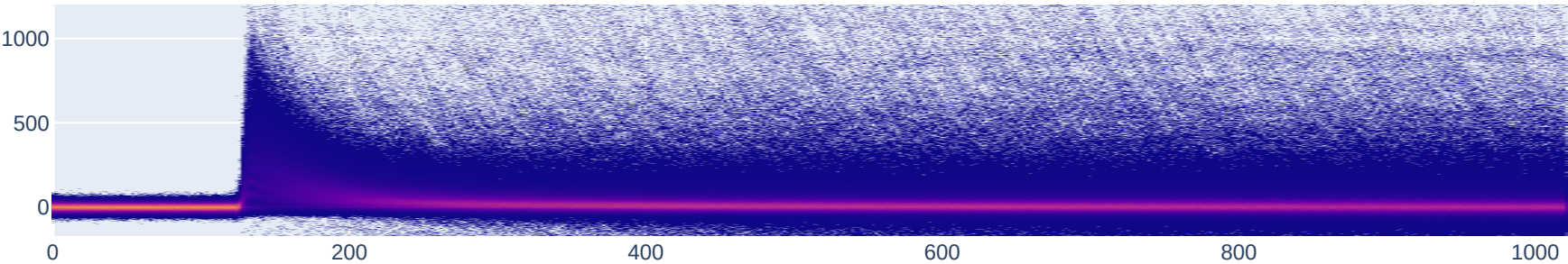
Persistence – Baseline std cut: 10779 wfs
