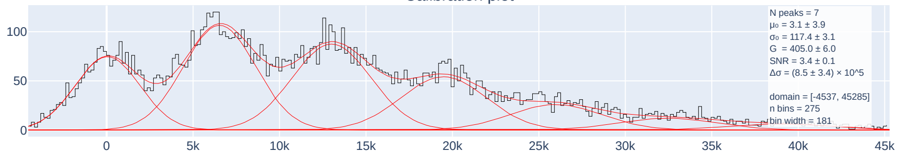
Calibration plot
