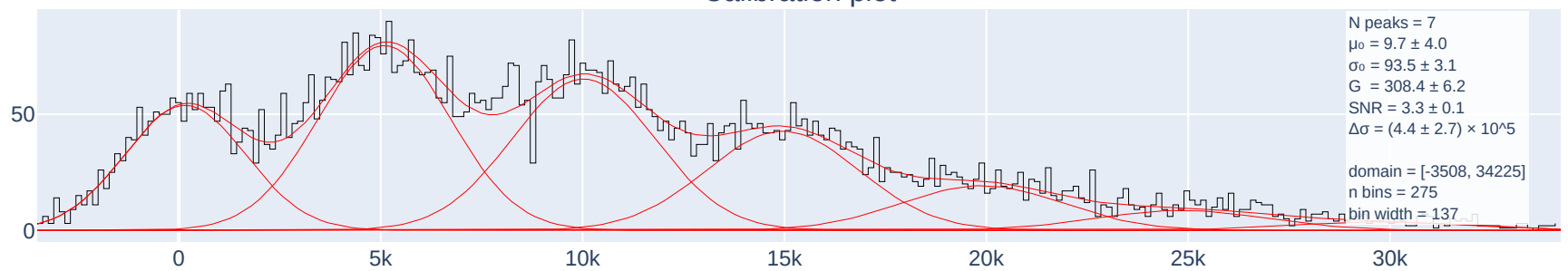
Calibration plot
