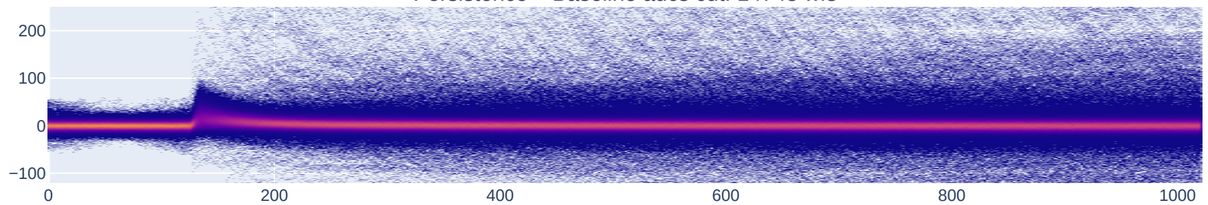
Persistence – Baseline adcs cut: 14743 wfs
