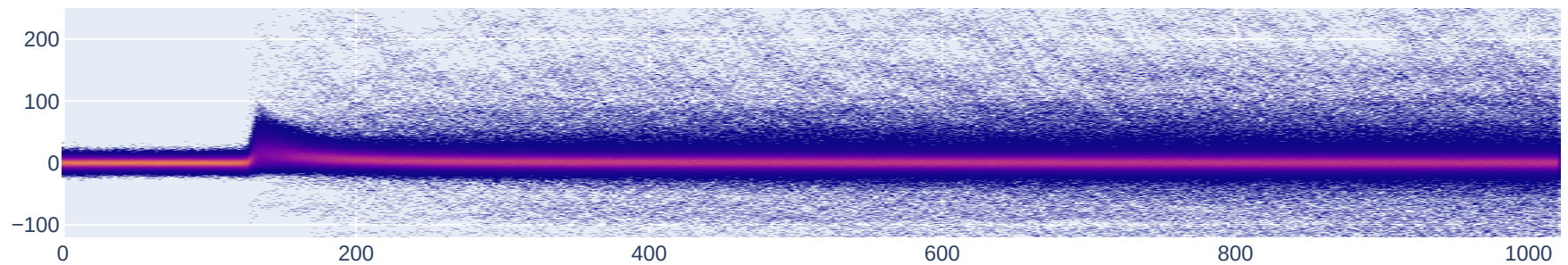
Persistence – Baseline std cut: 9219 wfs
