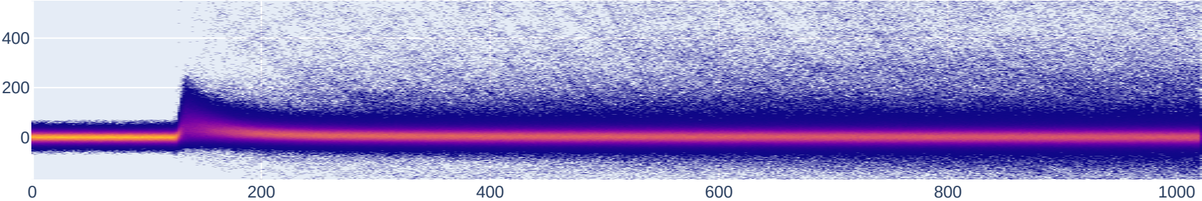
Persistence – Baseline std cut: 9520 wfs
