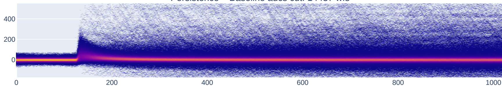
Persistence – Baseline adcs cut: 14437 wfs
