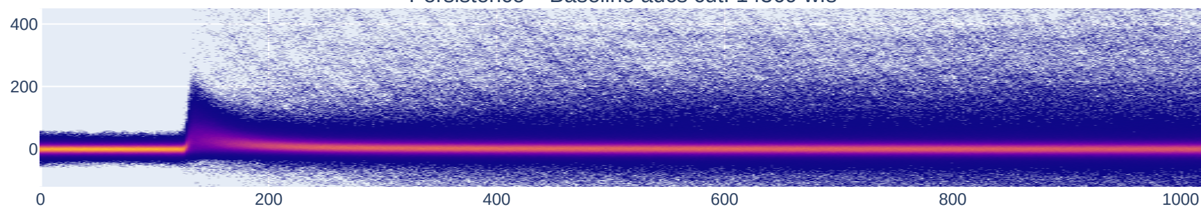
Persistence – Baseline adcs cut: 14369 wfs
