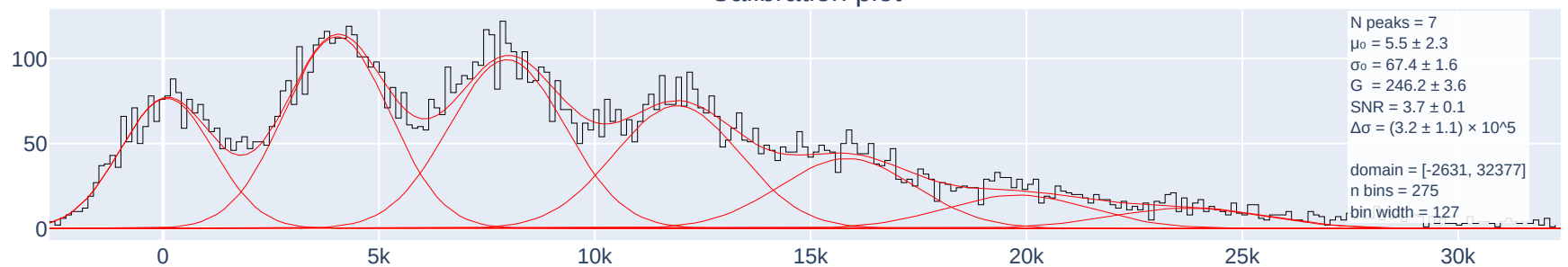
Calibration plot
