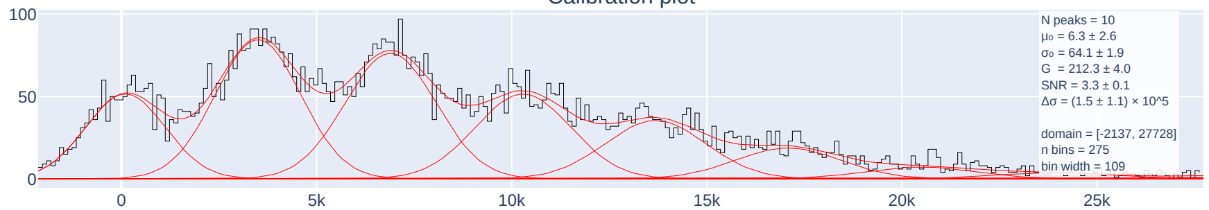
Calibration plot
