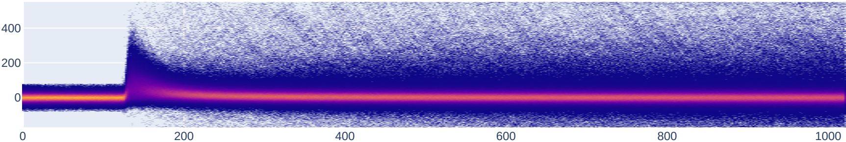
Persistence – Baseline adcs cut: 13525 wfs
