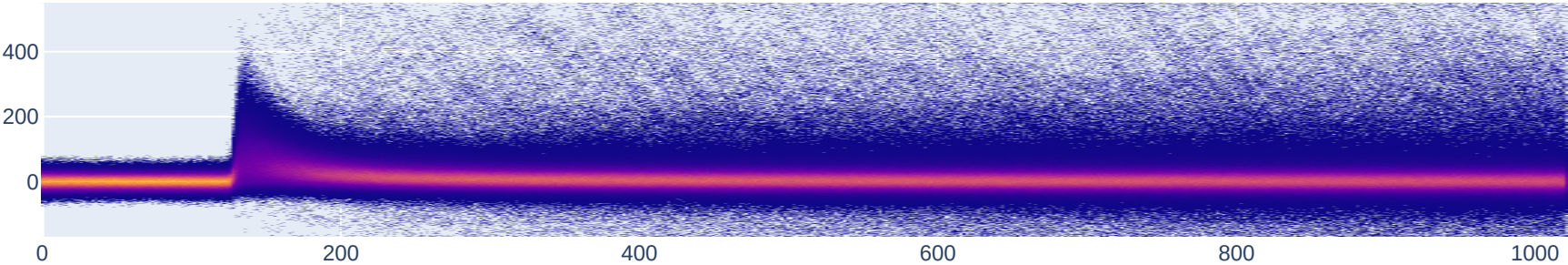
Persistence – Baseline std cut: 11161 wfs
