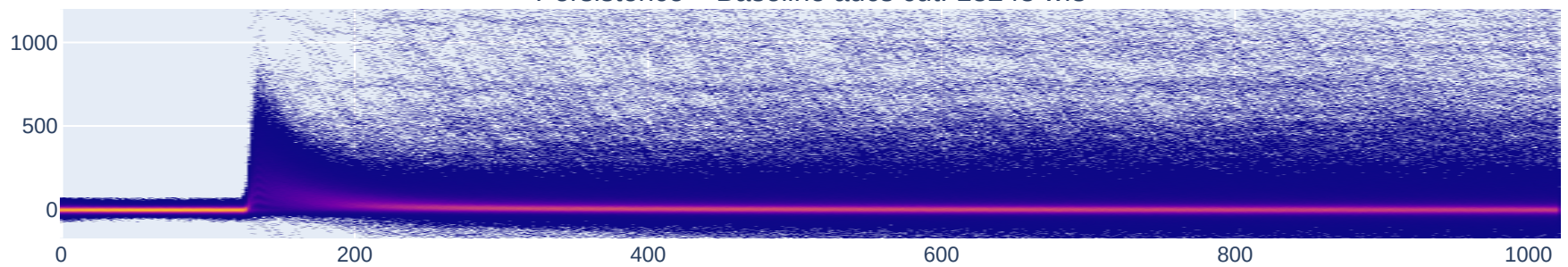
Persistence – Baseline adcs cut: 13243 wfs
